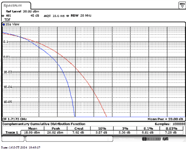
Band4-15MHz-16QAM-20025-25RB#0
