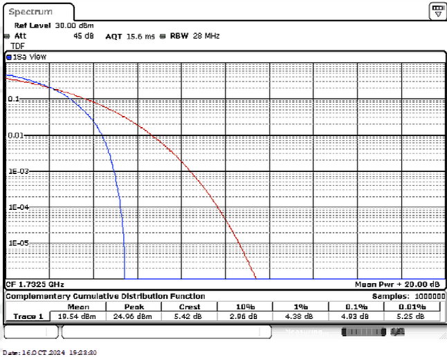
Band4-5MHz-16QAM-20175-25RB#0
