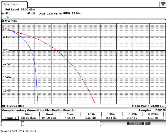
Band4-5MHz-QPSK-20175-25RB#0
