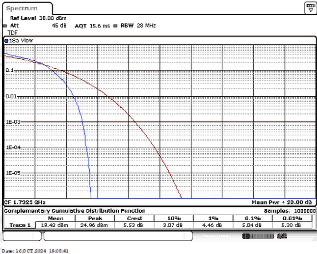
Band4-1.4MHz-16QAM-20175-6RB#0
