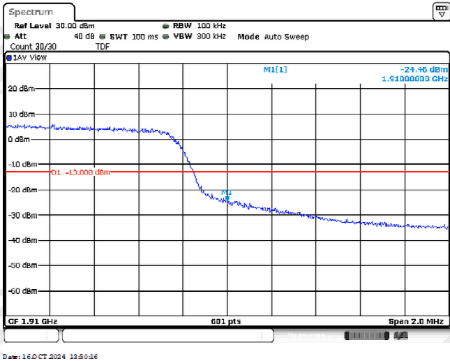
Band2-5MHz-QPSK-19175-25RB#0
