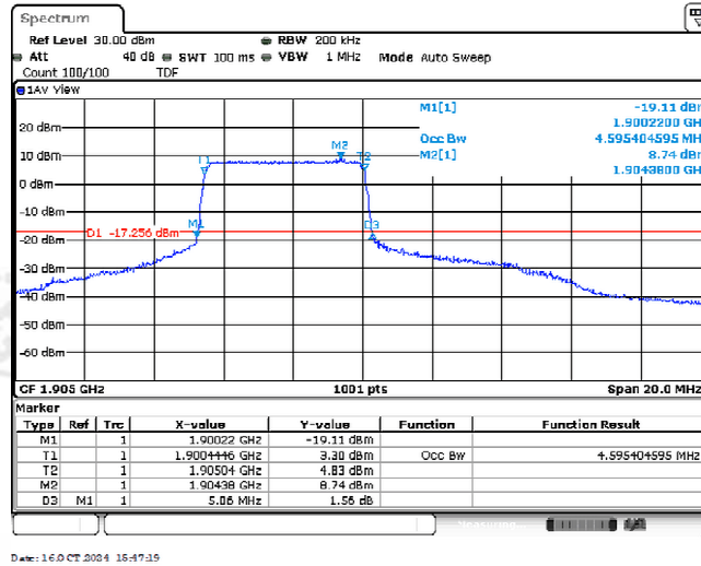
Band2-10MHz-16QAM-19150-25RB#0-4.595
