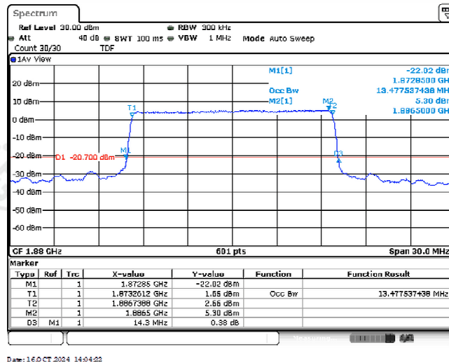
Band2-15MHz-QPSK-18900-75RB#0-13.478
