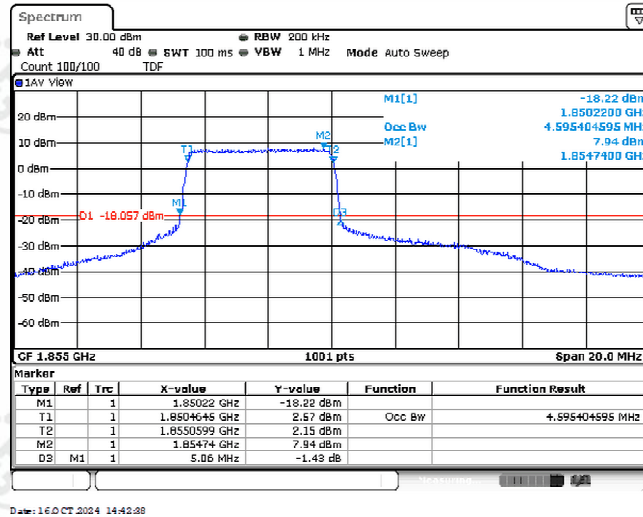
Band2-10MHz-16QAM-18650-25RB#0-4.595
