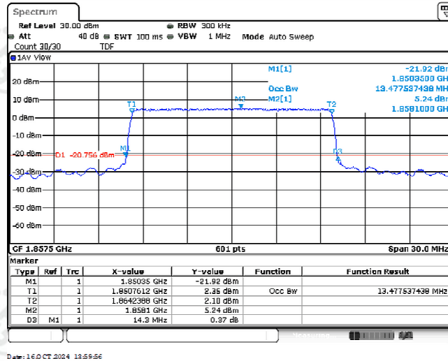
Band2-15MHz-QPSK-18675-75RB#0-13.478
