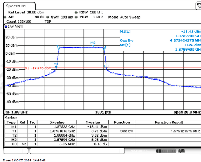
Band2-10MHz-16QAM-18900-25RB#0-4.575
