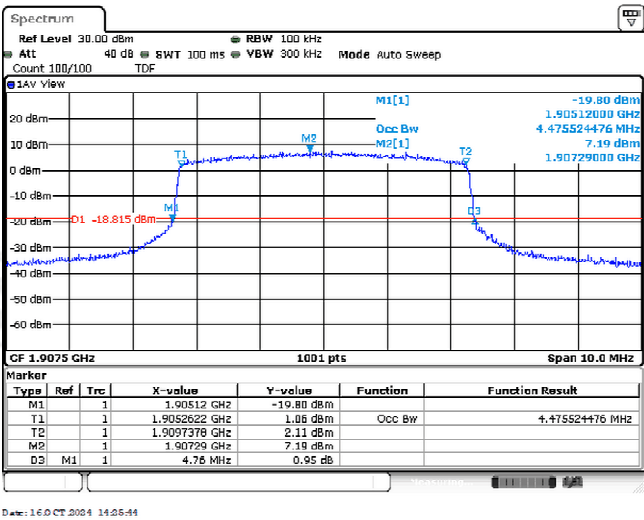
Band2-5MHz-16QAM-19175-25RB#0-4.476
