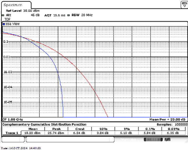
Band2-10MHz-16QAM-18900-25RB#0
