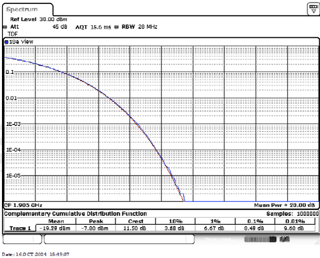
Band2-10MHz-16QAM-19150-25RB#0
