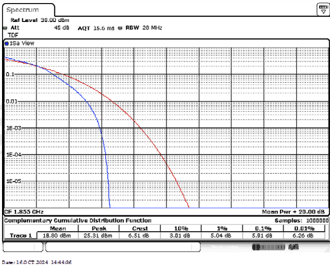
Band2-10MHz-16QAM-18650-25RB#0
