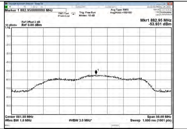
Cellular band DL
