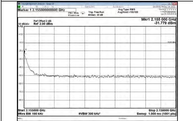
AWS Band LTE DL Right Side Pre AGC
