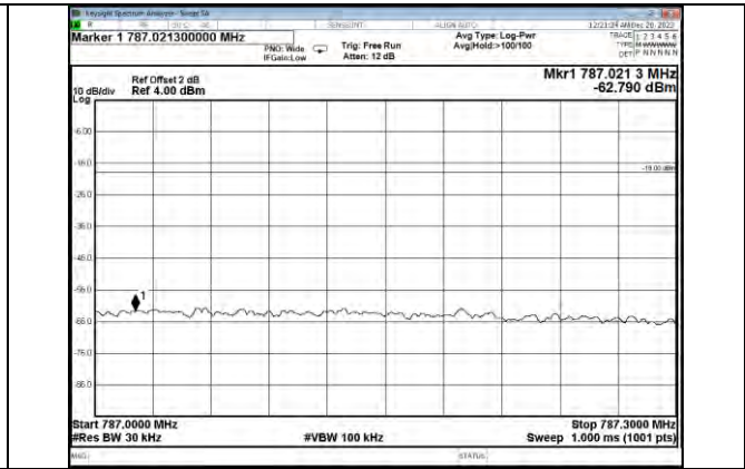
Upper 700MHz band CDMA UL Right Side 10dB Above AGC
