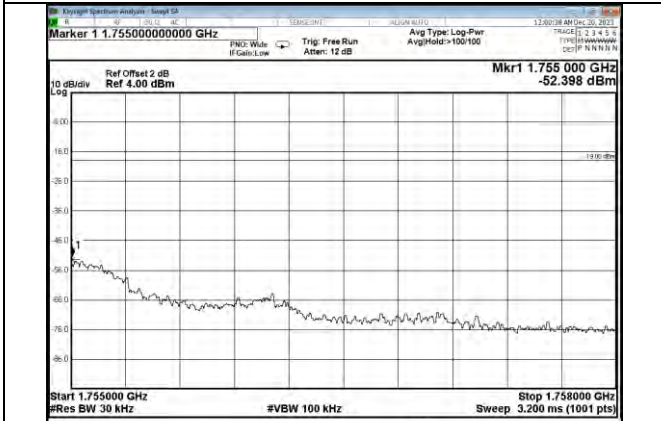
AWS Band CDMA UL Right Side Pre AGC
