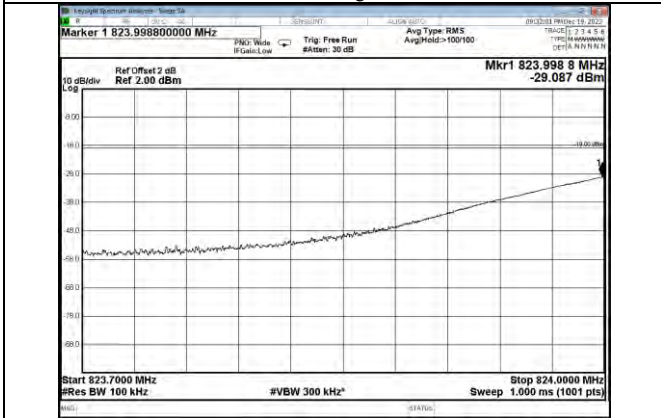
Cellular Band LTE UL Left Side Pre AGC
