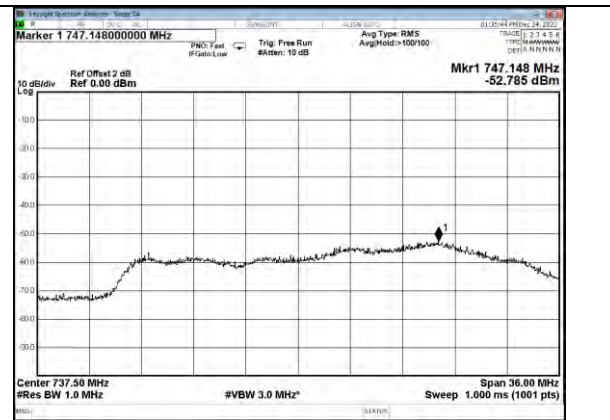
Lower 700MHz band DL
