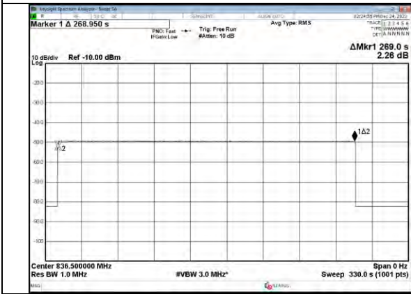
Cellular band
