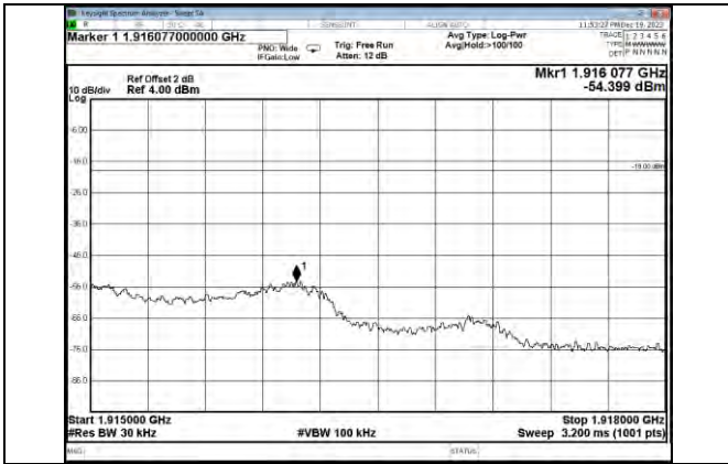
PCS Band CDMA UL Right Side Pre AGC
