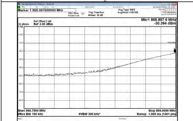
Cellular Band LTE DL Left Side Pre AGC
