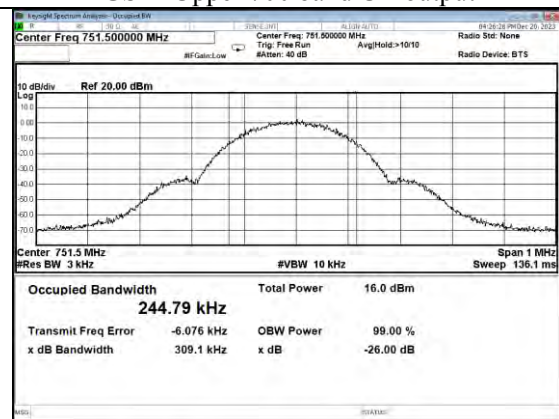
GSM-Upper 700 band DL output
