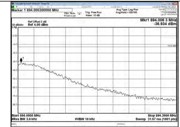
Cellular Band GSM DL Right Side 10dB Above AGC
