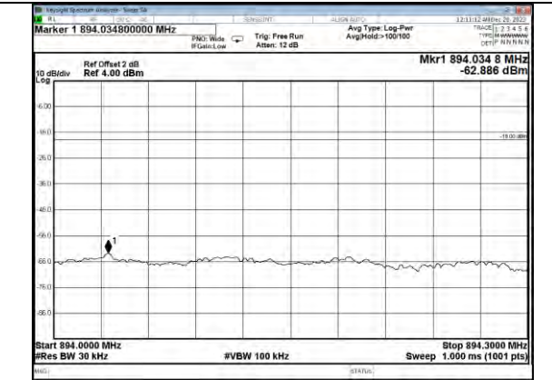
Cellular Band CDMA DL Right Side 10dB Above AGC
