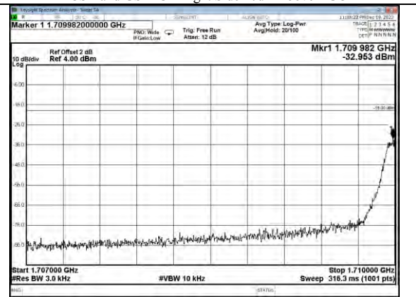
AWS Band GSM UL Left Side 10dB Above AGC
