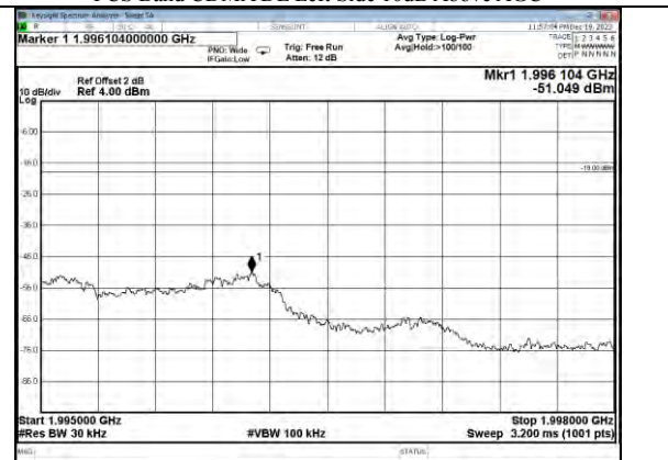
PCS Band CDMA DL Right Side 10dB Above AGC
