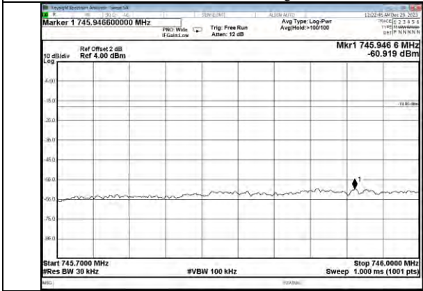
Upper 700MHz band CDMA DL Left Side Pre AGC
