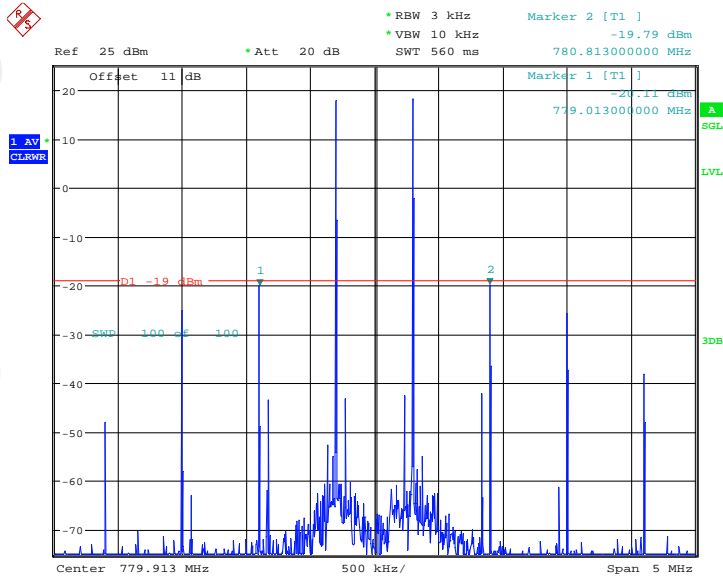
Band13 AGC +10dB, UL
