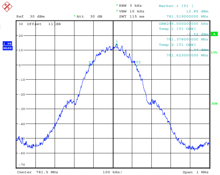
Band13 GSM UL output
