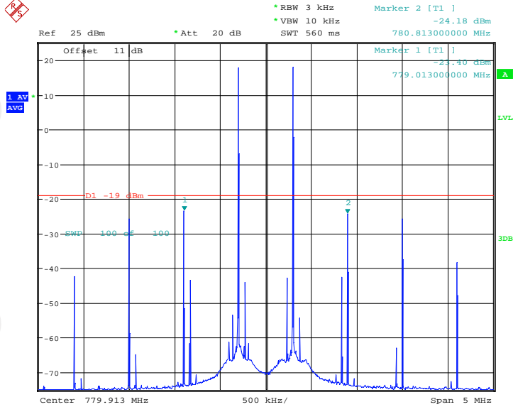
Band13 Pre AGC, UL
