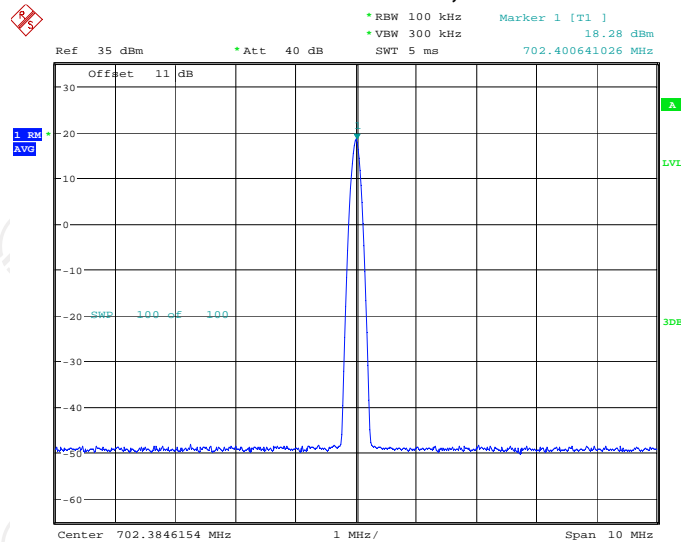
Band12 CW, UL
