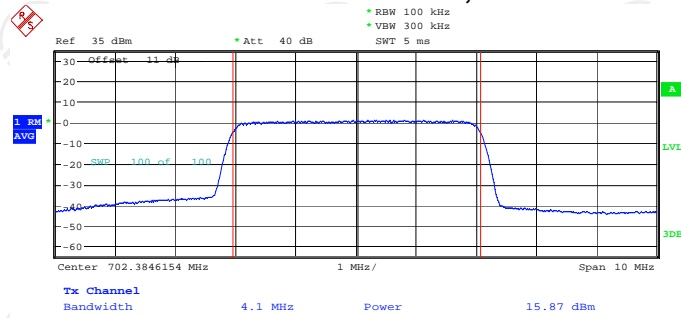
Band12 AWGN, UL
