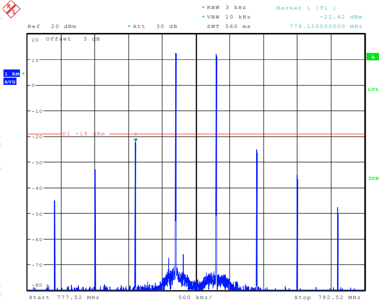
Band13 AGC +10dB, UL
