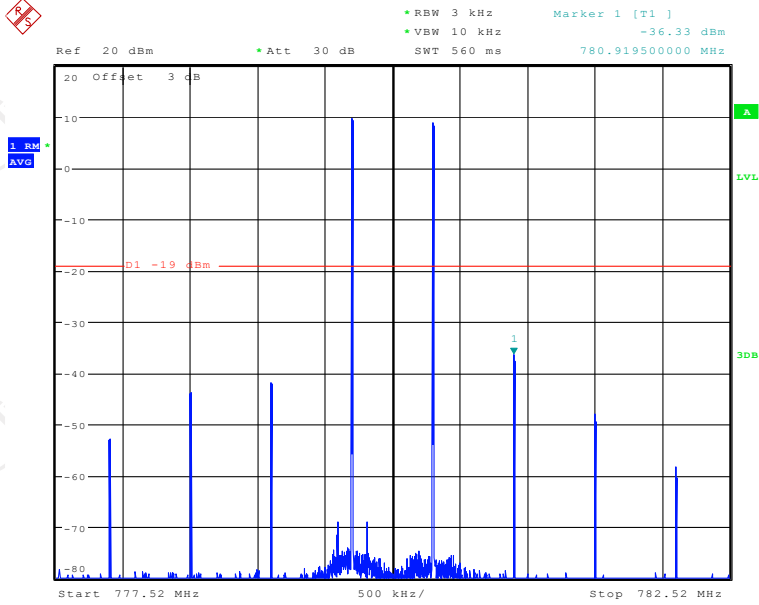
Band13 Pre AGC, UL
