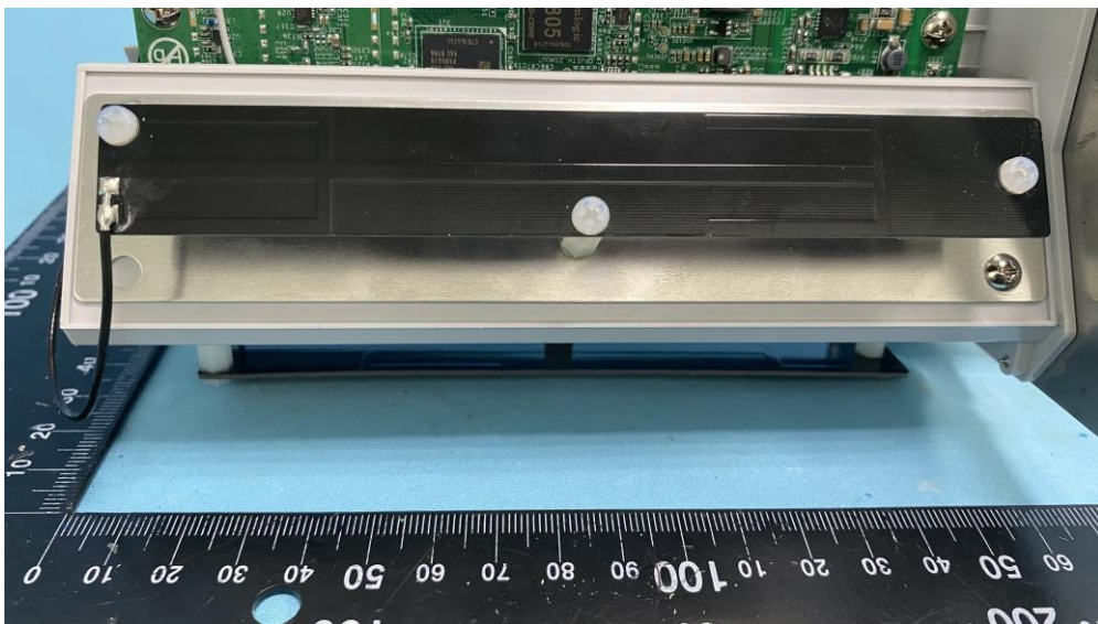
(12) EUT Photo (BLE Internal Antenna)
