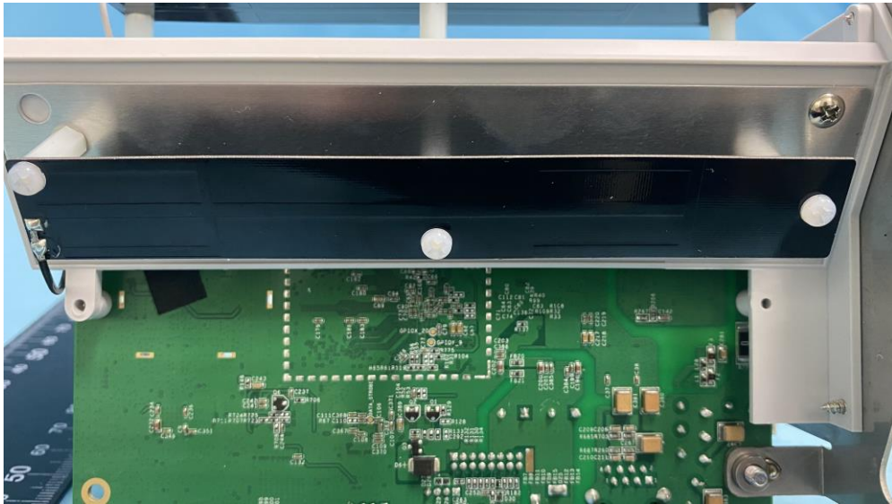
(11) EUT Photo (BLE Internal Antenna)
