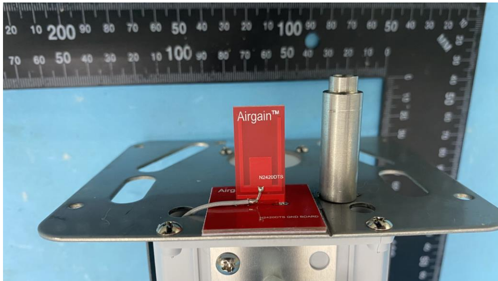
(15) EUT Photo (Wi-Fi Antenna)
