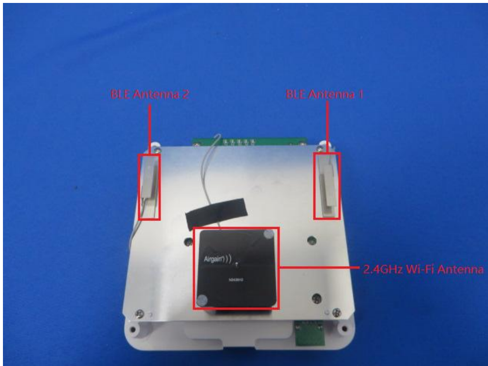
(4) EUT Photo (BLE Antenna 2 can't transmit declared by the applicant)
