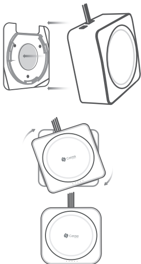
Installation Murale
