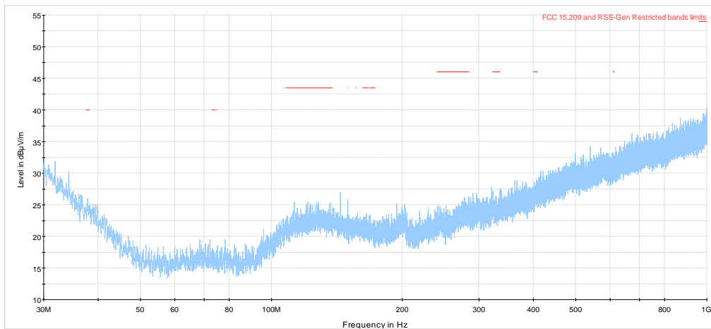
NEX-455174 RE 30-1000 MHz WiFi 802.11b Mid ch Preview Result 1-PK+ FCC 15.209 and RSS-Gen Restricted bands limits
