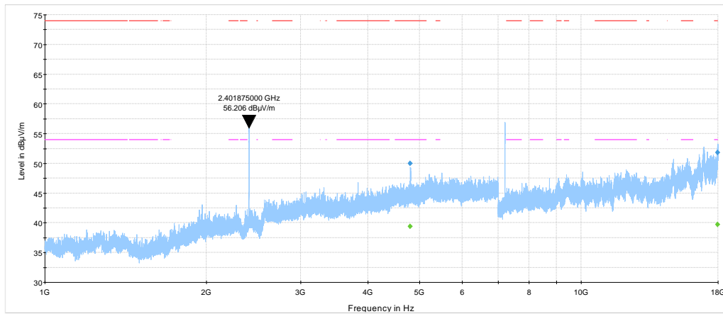
NEX-455174 RE 1-18 GHz - BLE - Low channel Preview Result 1-PK+ FCC 15.209 and RSS-Gen Restricted bands peak limits FCC 15.209 and RSS-Gen Restricted bands average limits Final_Result PK+ Final_Result CAV
