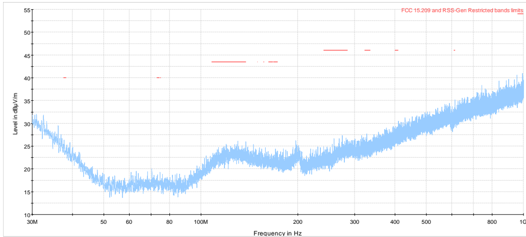
NEX-455174 RE 30-1000 MHz - BLE - High channel Preview Result 1-PK+ FCC 15.209 and RSS-Gen Restricted bands limits
