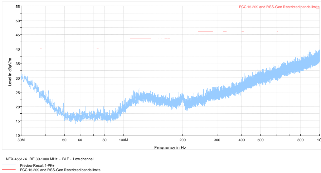
Figure 8.1-16: Radiated spurious emissions 30- 1000 MHz on Low ch
