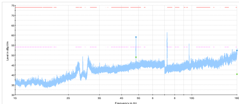
NEX-455174 RE, 1-18 GHz, WiFi 802.11b Low channel Preview Result 1-PK+ FCC 15.209 and RSS-Gen Restricted bands peak limits FCC 15.209 and RSS-Gen Restricted bands average limits Final_Result PK+ Final_Result CAV
