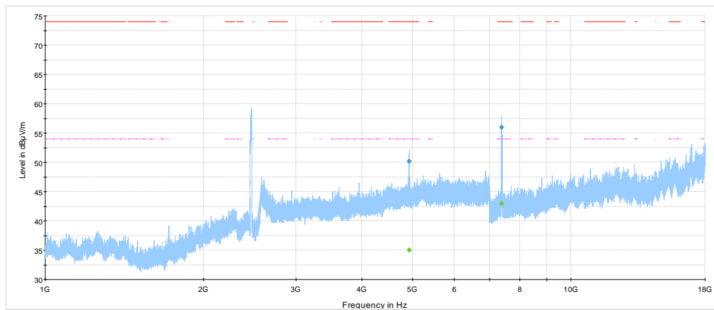
NEX-455174 RE, 1-18 GHz, WiFi 802.11g High channel — Preview Result 1-PK+ — FCC 15.209 and RSS-Gen Restricted bands peak limits — FCC 15.209 and RSS-Gen Restricted bands average limits ◆ Final_Result PK+ ◆ Final_Result CAV
