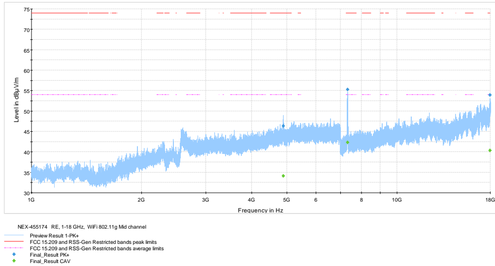
Figure 8.1-8: Radiated spurious emissions 1- 18 GHz on Mid ch
