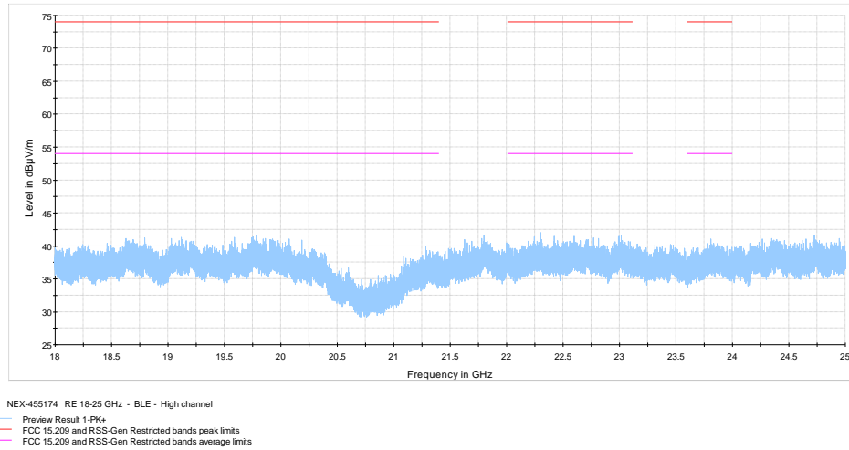
Figure 8.1-24: Radiated spurious emissions 18- 25 GHz on High ch
