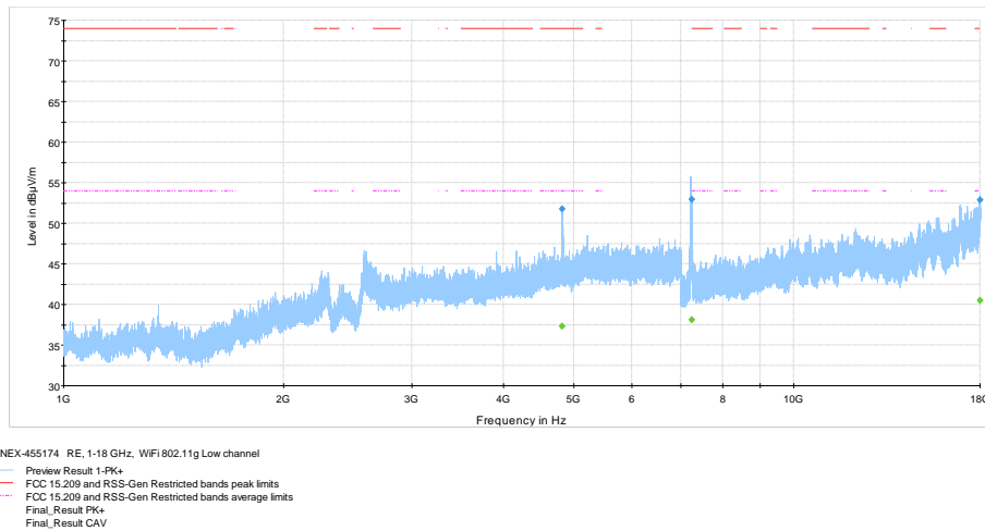
Figure 8.1-7: Radiated spurious emissions 1- 18 GHz on Low ch
