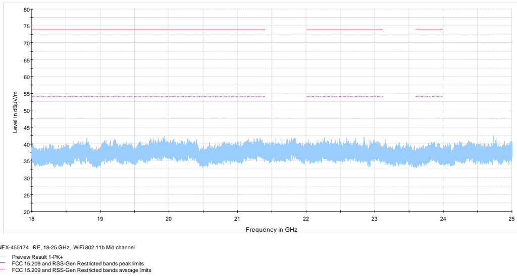
Figure 8.1-5: Radiated spurious emissions 18- 25 GHz on Mid ch, sample plot
