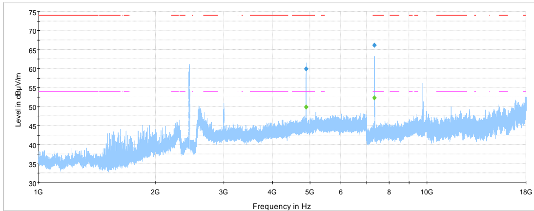
NEX-455174 RE, 1-18 GHz, WiFi 802.11b Mid channel — Preview Result 1-PK+ — FCC 15.209 and RSS-Gen Restricted bands peak limits — FCC 15.209 and RSS-Gen Restricted bands average limits ◆ Final_Result PK+ ◆ Final_Result CAV
