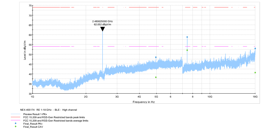
Figure 8.1-21: Radiated spurious emissions 1- 18 GHz on High ch
