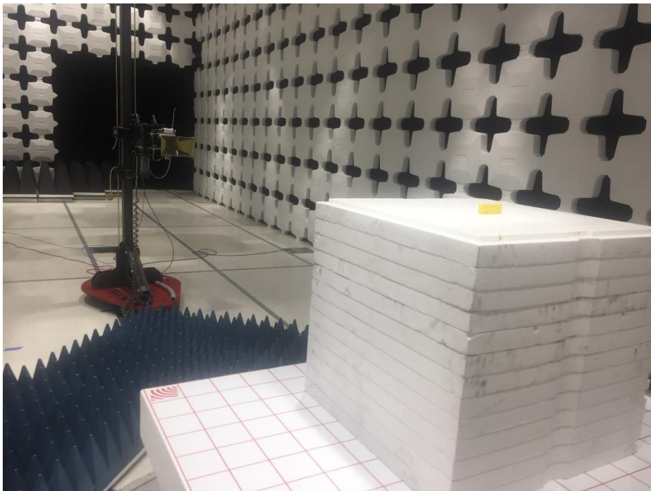
Radiated Emissions Above 1GHz setup – Rear (non-flex model)
