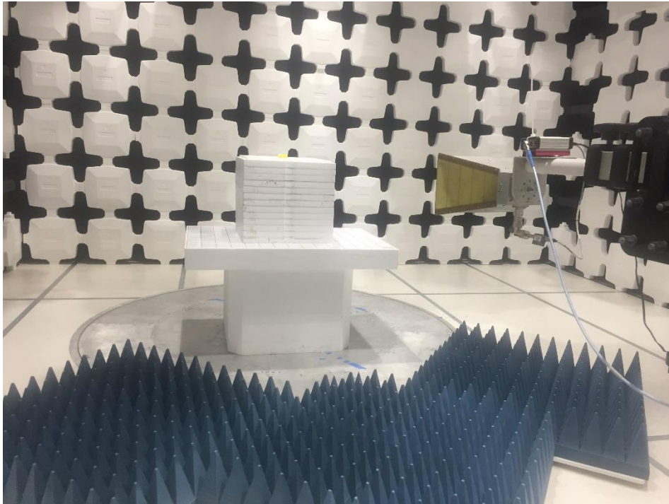
Radiated Emissions Above 1GHz setup – Front (non-flex model)
