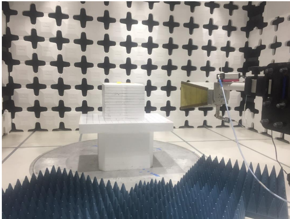
Radiated Emissions Above 1GHz setup – Front (flex model)
