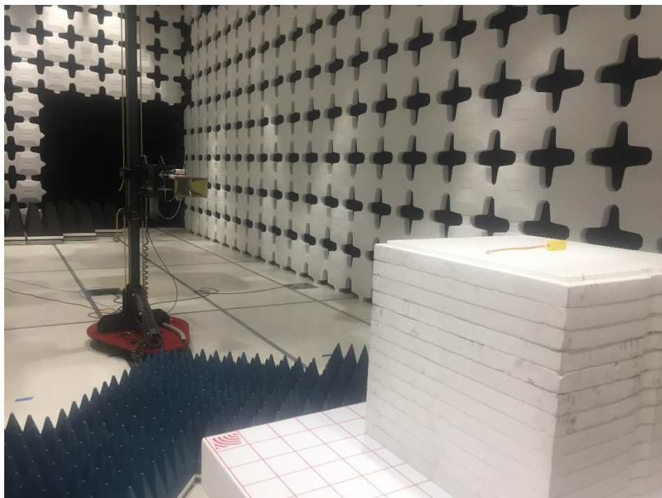
Radiated Emissions Above 1GHz setup – Rear (flex model)
