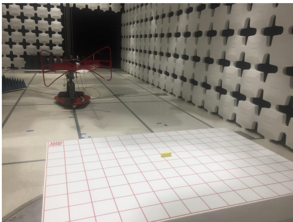
Radiated Emissions Below 1GHz setup – Rear (non-flex model)
