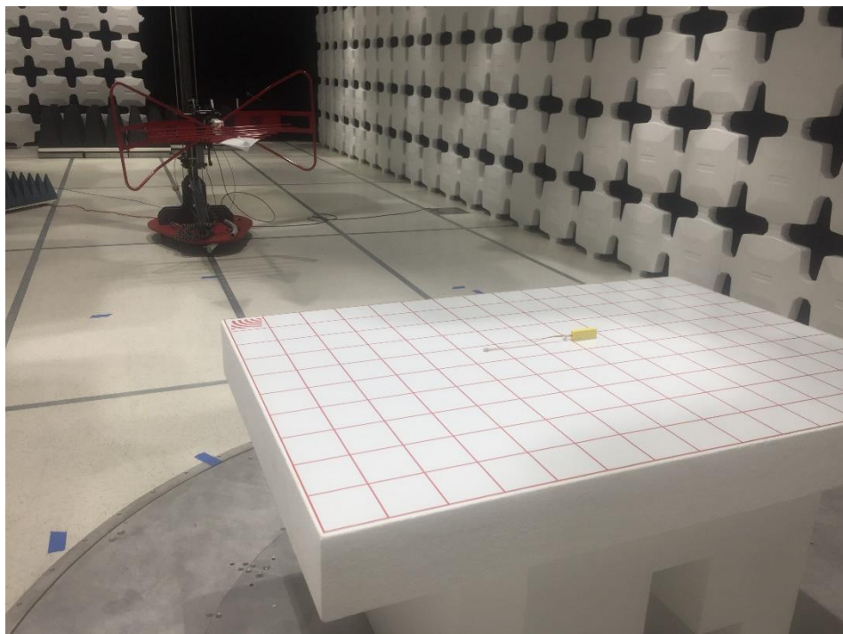
Radiated Emissions Below 1GHz setup – Rear (flex model)
