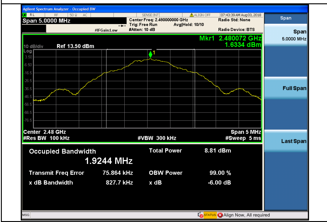
BLE-2480MHz-2Mbps
