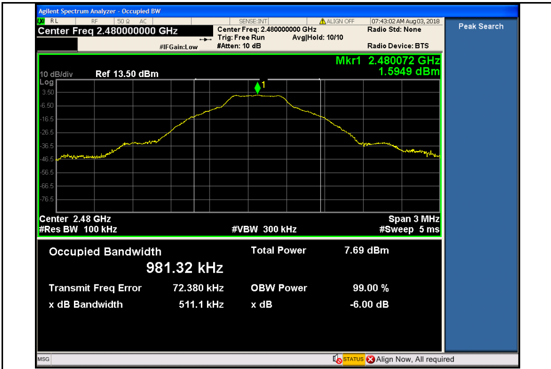
BLE-2480MHz-1Mbps
