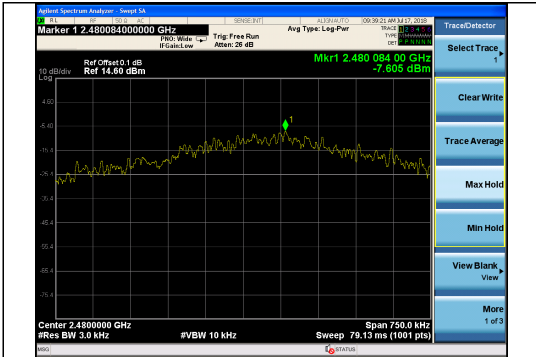
BLE-2480MHz-1Mbps
