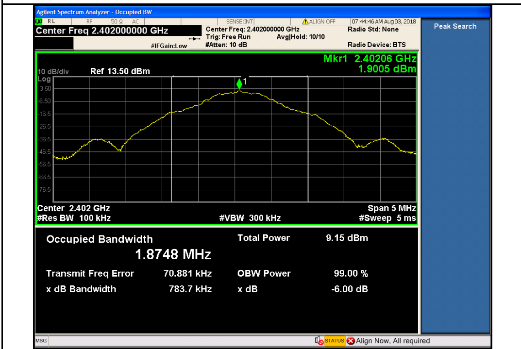
BLE-2402MHz-2Mbps
