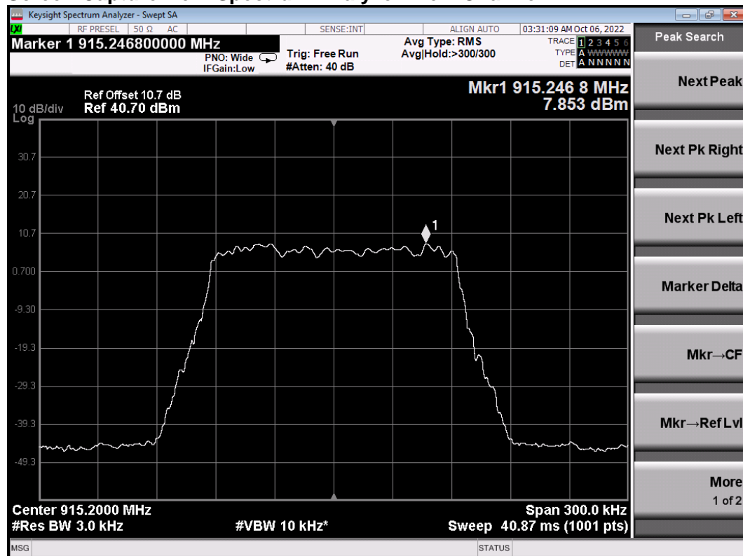
Screen Capture from Spectrum Analyzer: Low Channel
