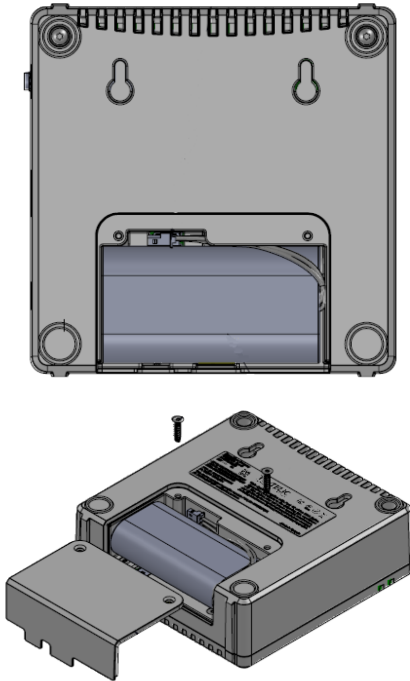
Figure 12: Battery Installation
