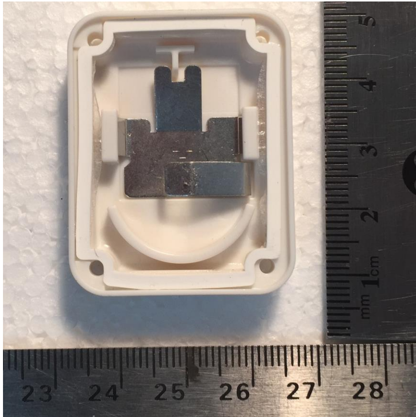
T0007376 inside enclosure with battery
