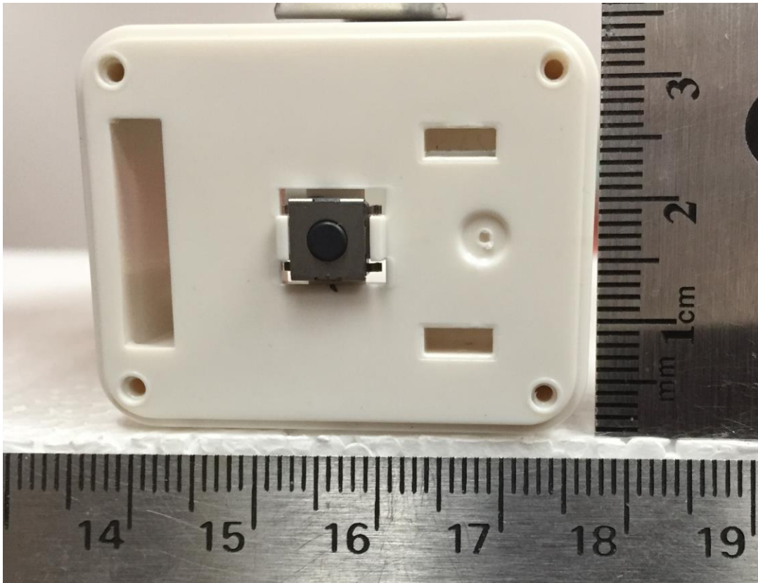
T0007376 rear enclosure
