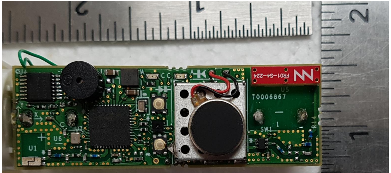
T0007126 PCBA top without vibration actuator
