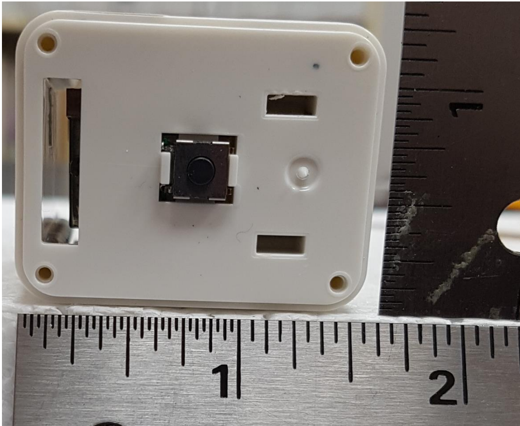
T0007125 rear cover (button)
