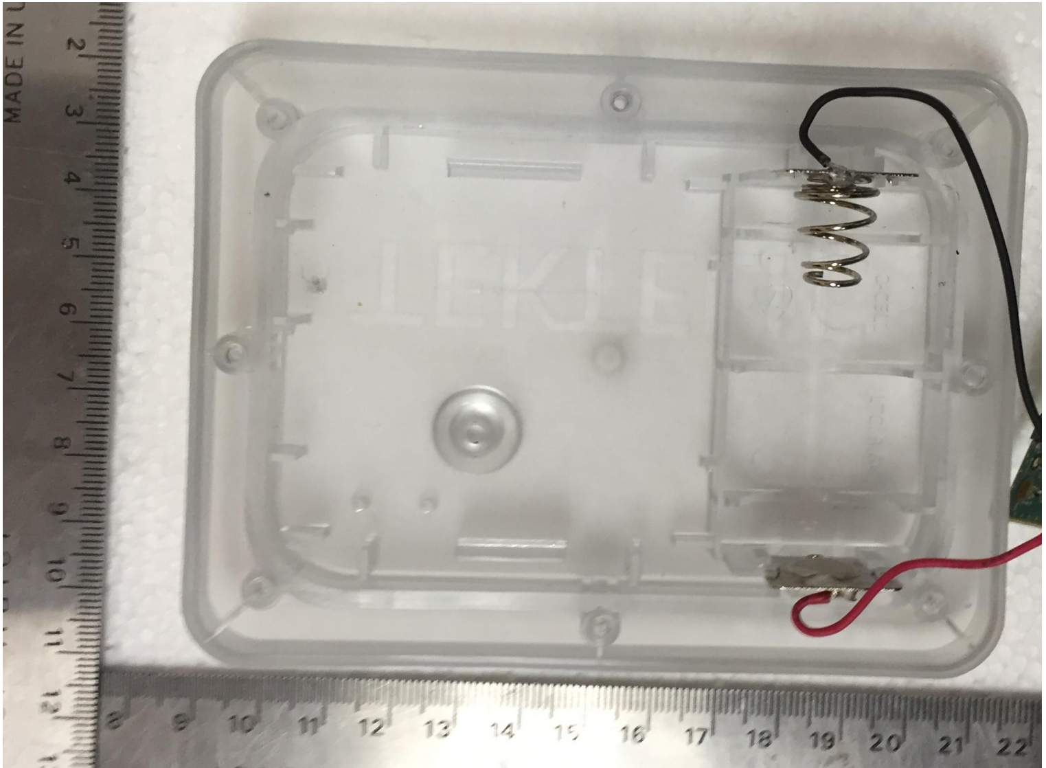
Top Cover inside view (T0005986 Variant)
