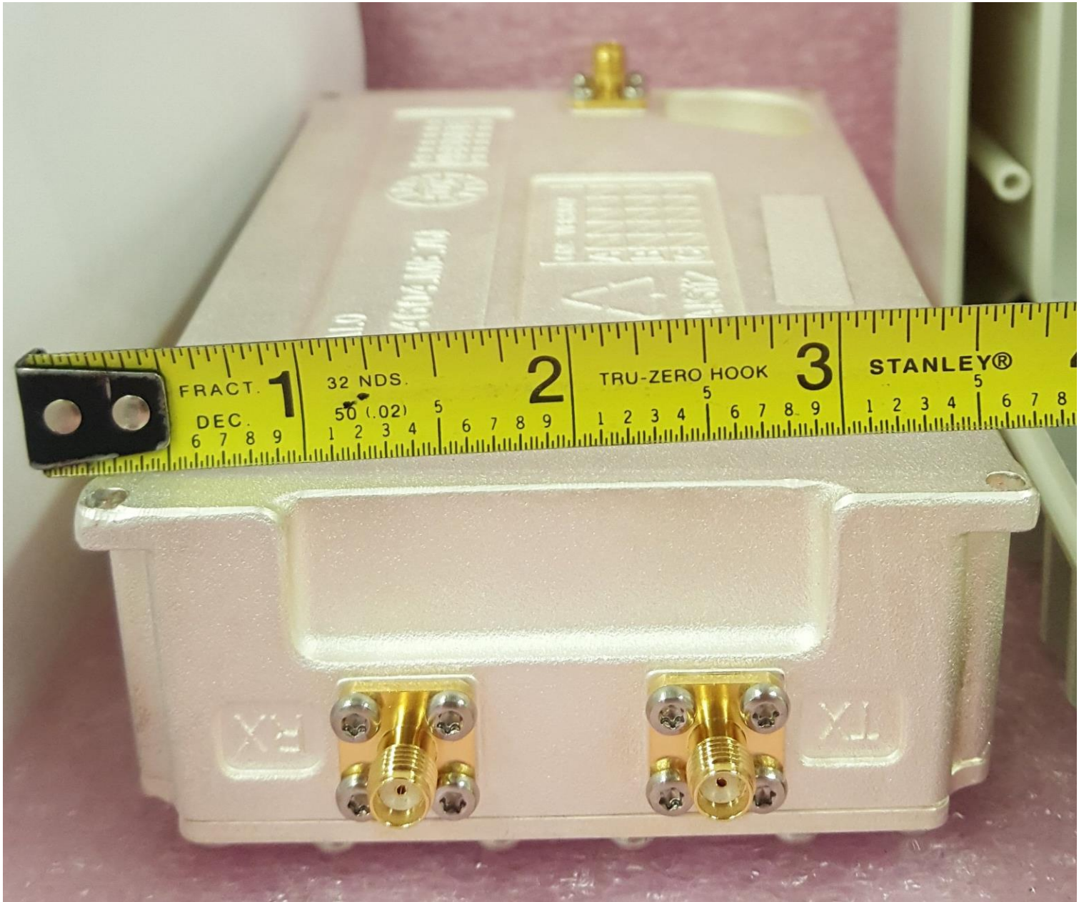
EUT Mechanical: duplexer view bottom front
