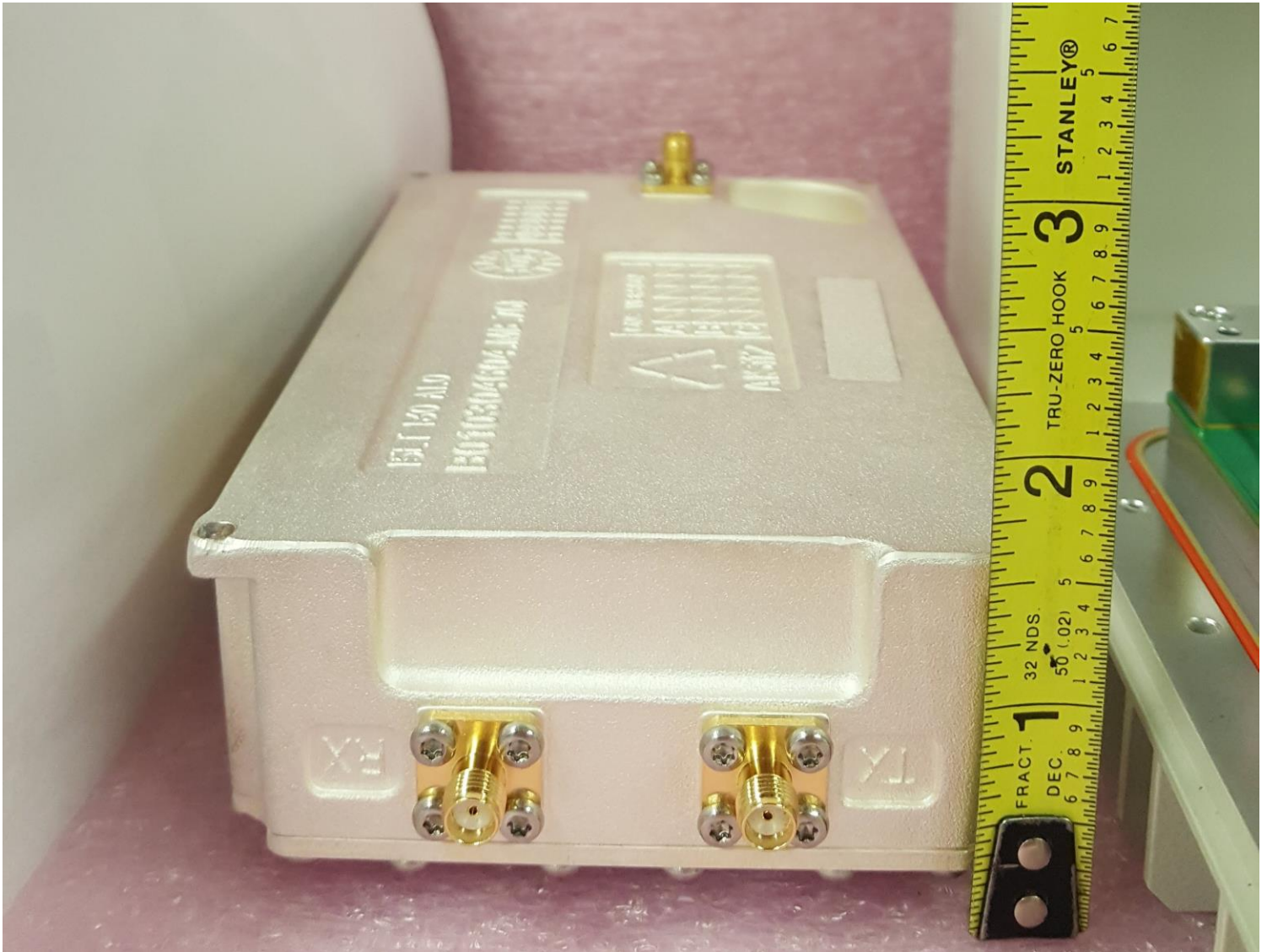
EUT Mechanical: duplexer view bottom
