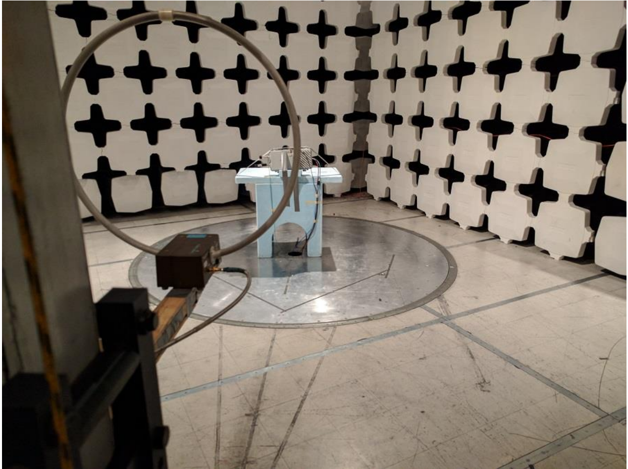
Radiated Emission below 30MHz Test Setup
