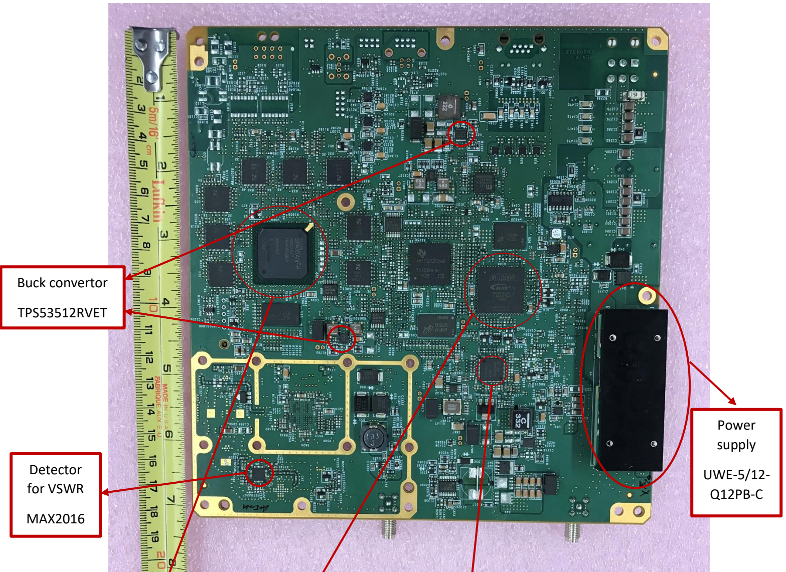
Figure 8 Gen 1 Mobile gateway secondary side
