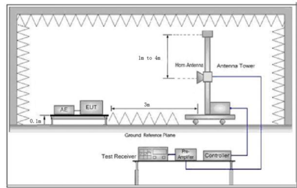
Figure 3. Above 1 GHz
