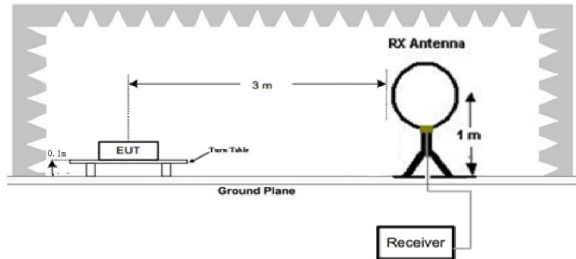
Figure 1. Below 30MHz
