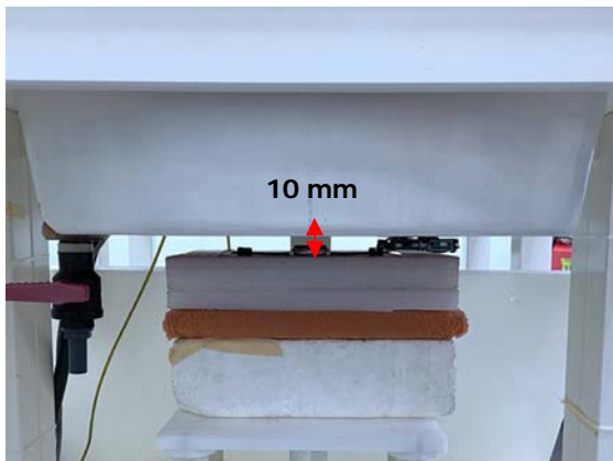
Fig.6 Front side of EUT (Rubber) to flat phantom
