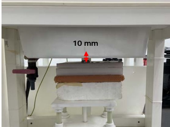
Fig.5 Front side of EUT (Matel) to flat phantom
