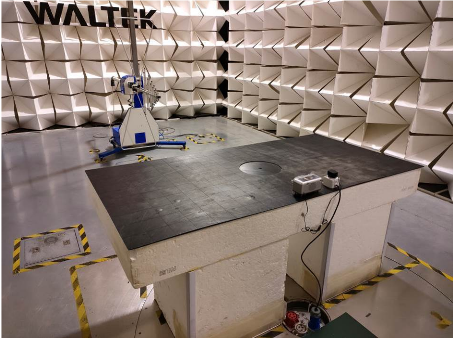
For 30MHz-1000MHz Test Site 1#
