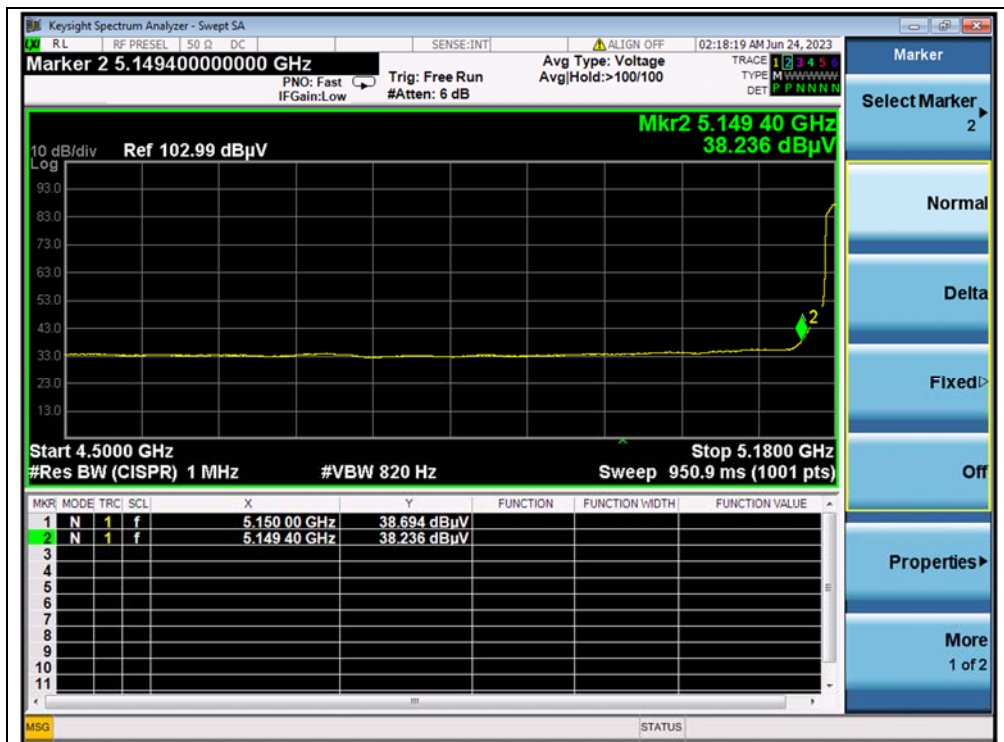
(AVERAGE, Channel 36, 802.11n (HT20))
