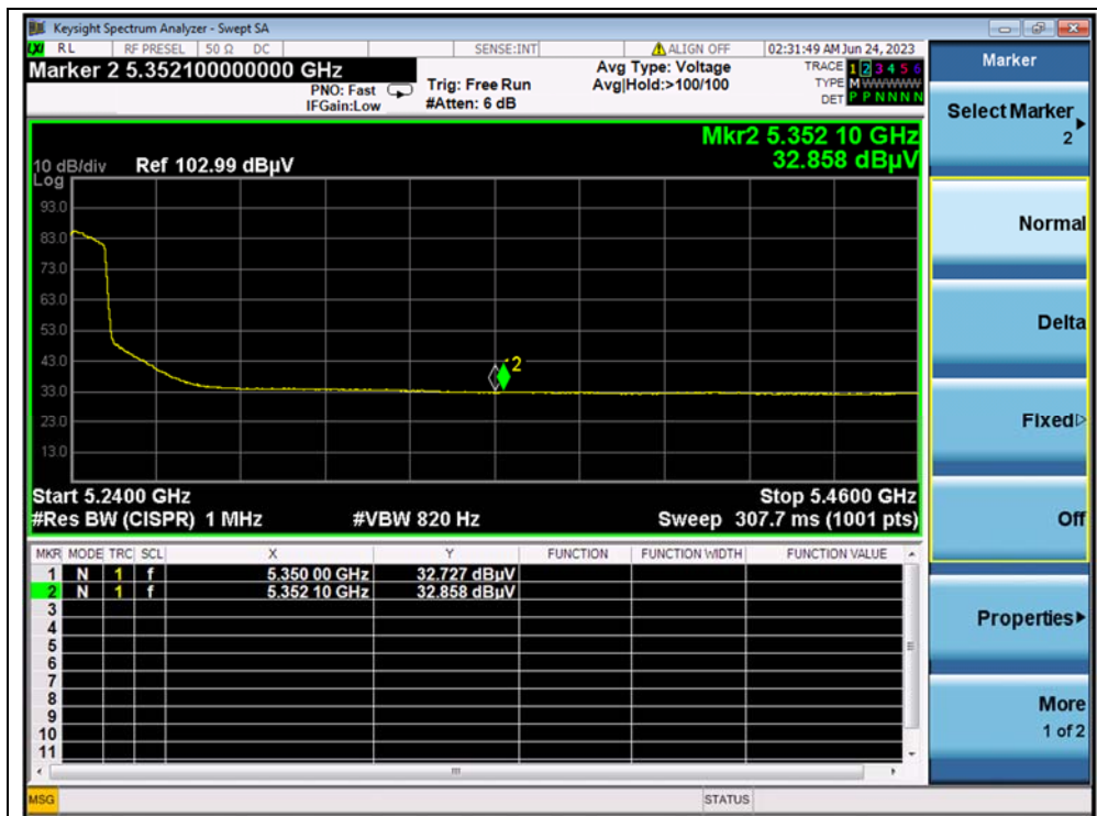
(AVERAGE, Channel 48, 802.11n (HT20))
