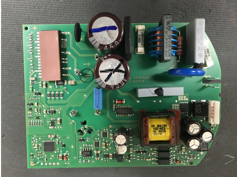
Motor Assembly PCB – Component Side
