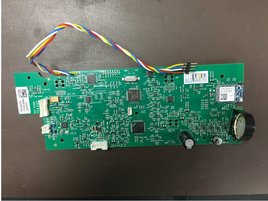
Control Board Assembly PCB – Component Side
