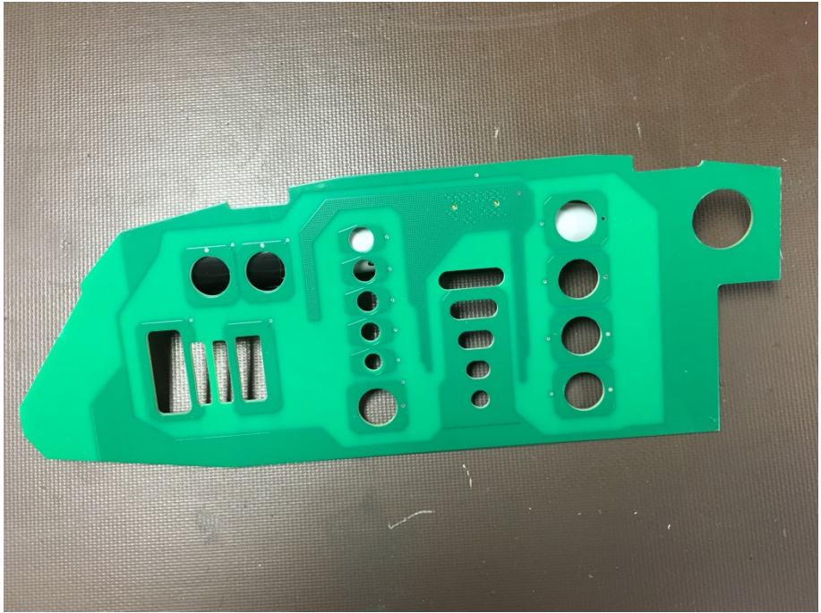
Touch Board Assembly – Trace Side
