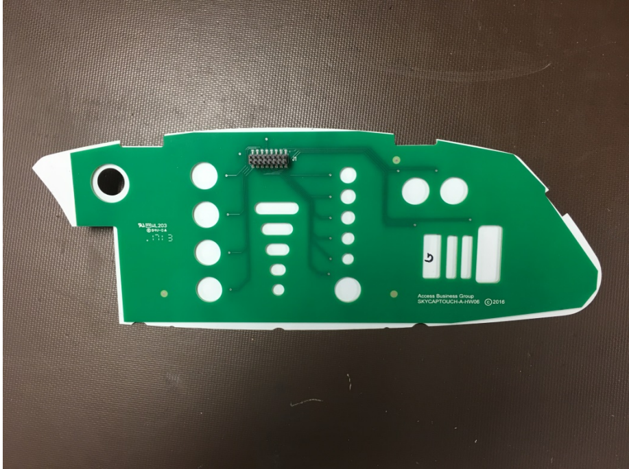
Touch Board Assembly – Connector Side
