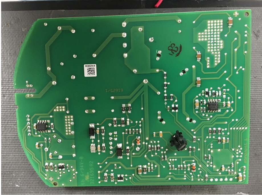
Motor Assembly PCB – Trace Side
