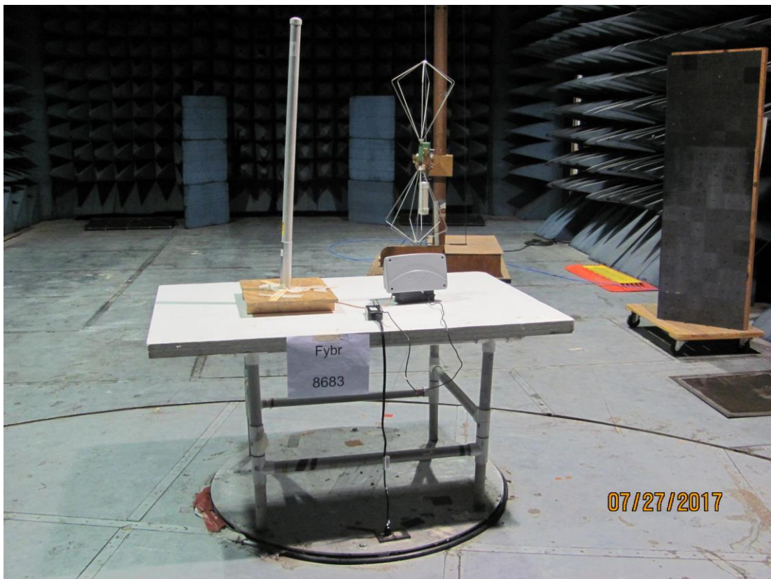
Omnidirectional Antenna
