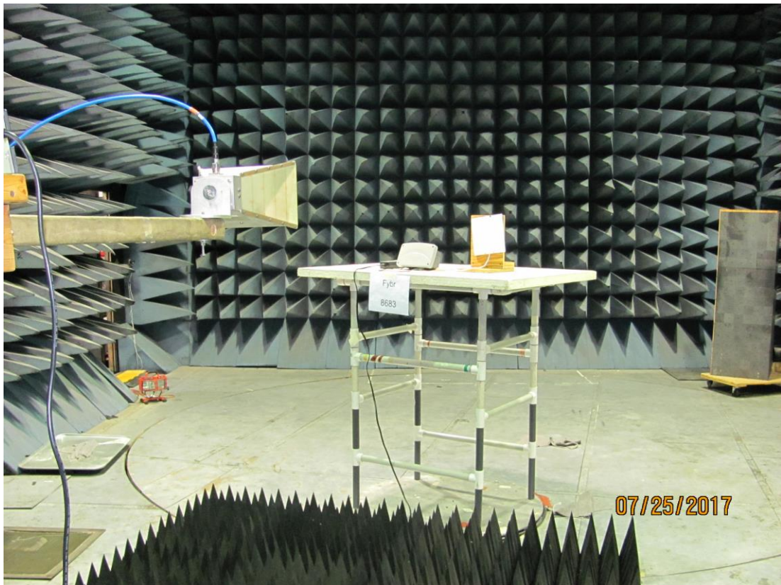
Patch Antenna
