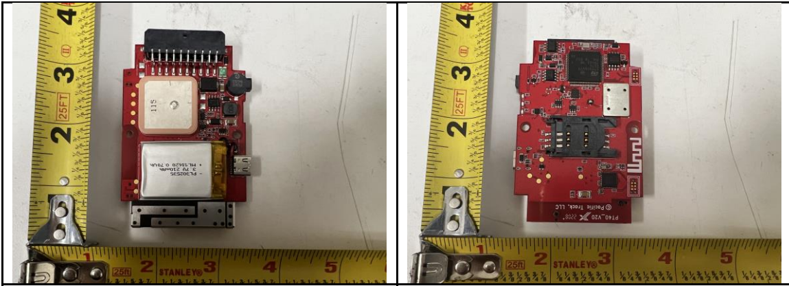
Mainboard_Front View
