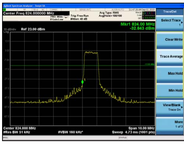
LTE Band 26 16QAM 1.4MHz CH-Low 100%RB
