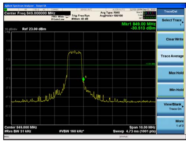
LTE Band 26 16QAM 1.4MHz CH-High 100%RB
