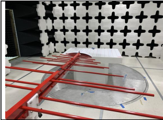
Radiated Emission Test below 1GHz Front View
