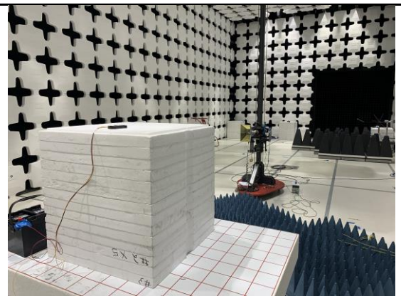
Radiated Emission Test above 1GHz Rear View
