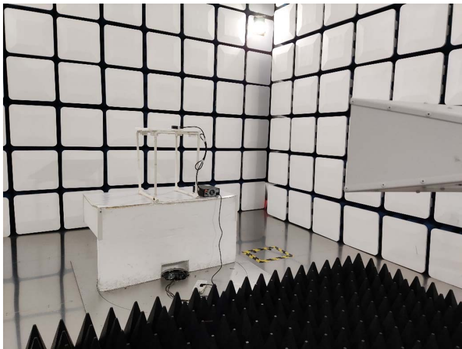
Above 1GHz-BLE
