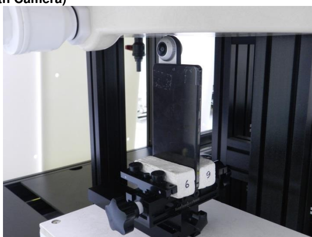
Top side with 0 mm separation distance (Phone with Camera)
