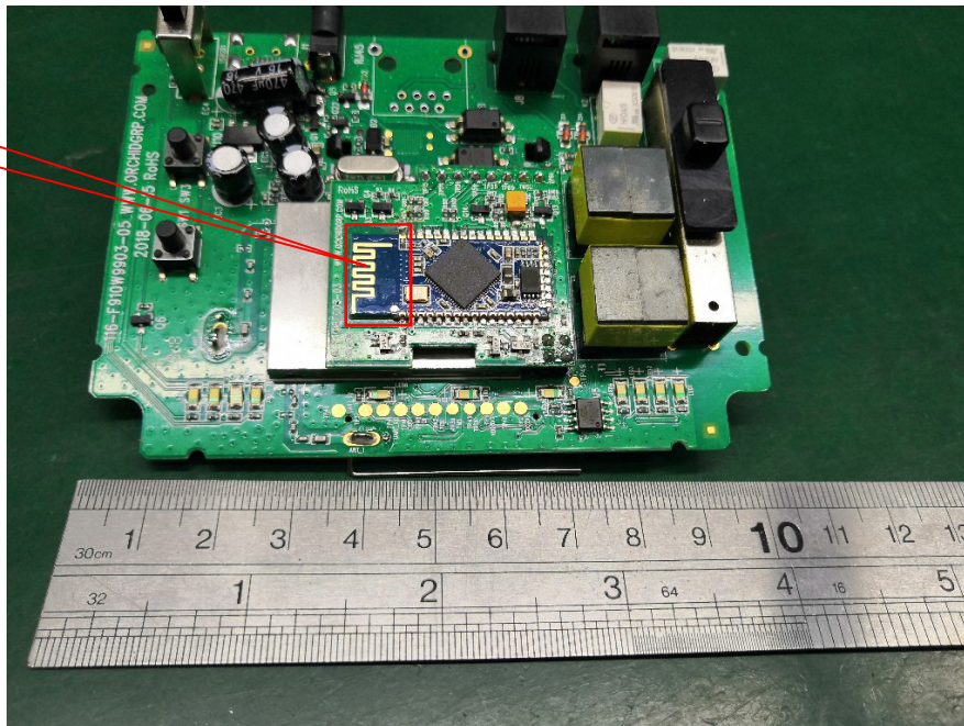
EUT – Main Board Top View 2 (Shielding off)
