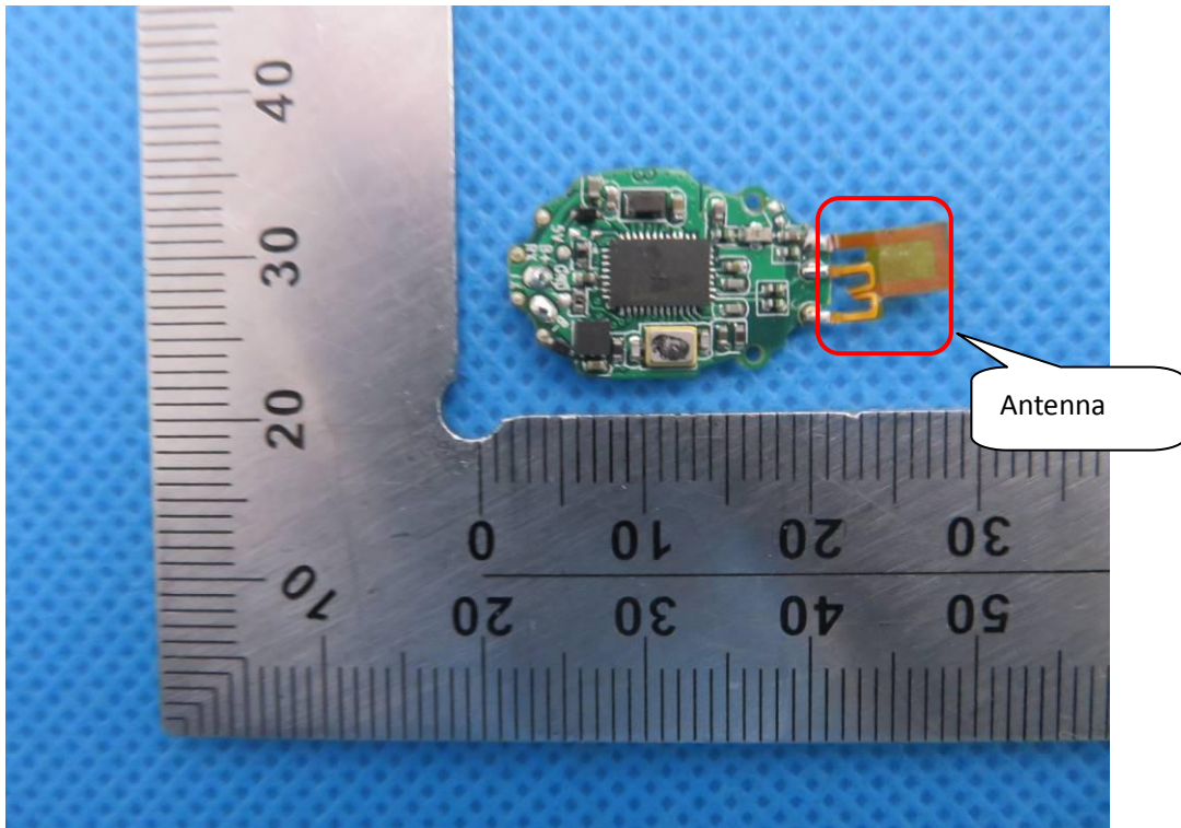
INTERNAL VIEW OF EUT(left)-1
