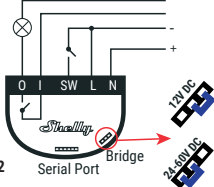
Power supply: 12V; 24-60V DC
