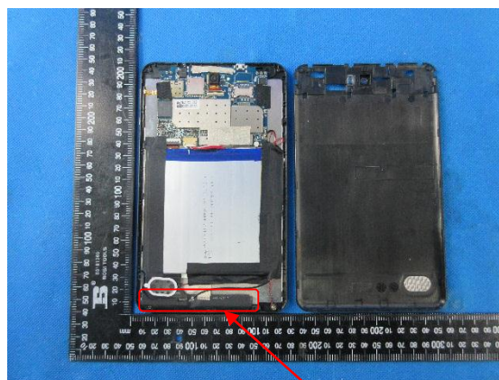
GSM/WCDMA/LTE Main ANT
