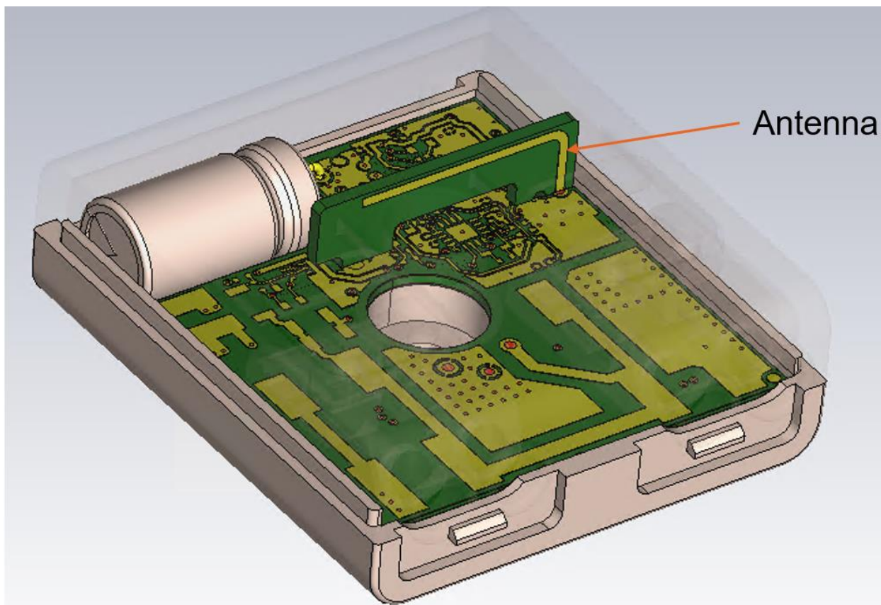
Figure 4: Antenna location in CBU-TED-LR
