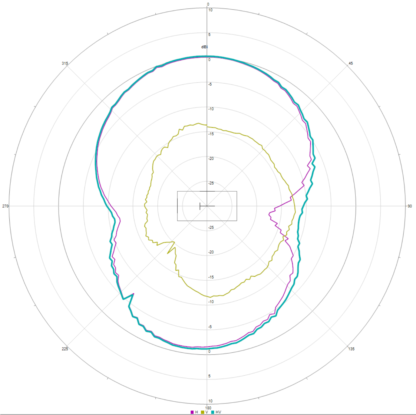
Figure 3: Radiation Pattern - XY-plane
