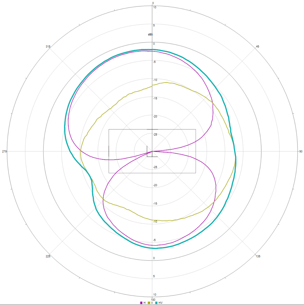
Figure 1: Radiation Pattern - YZ-plane
