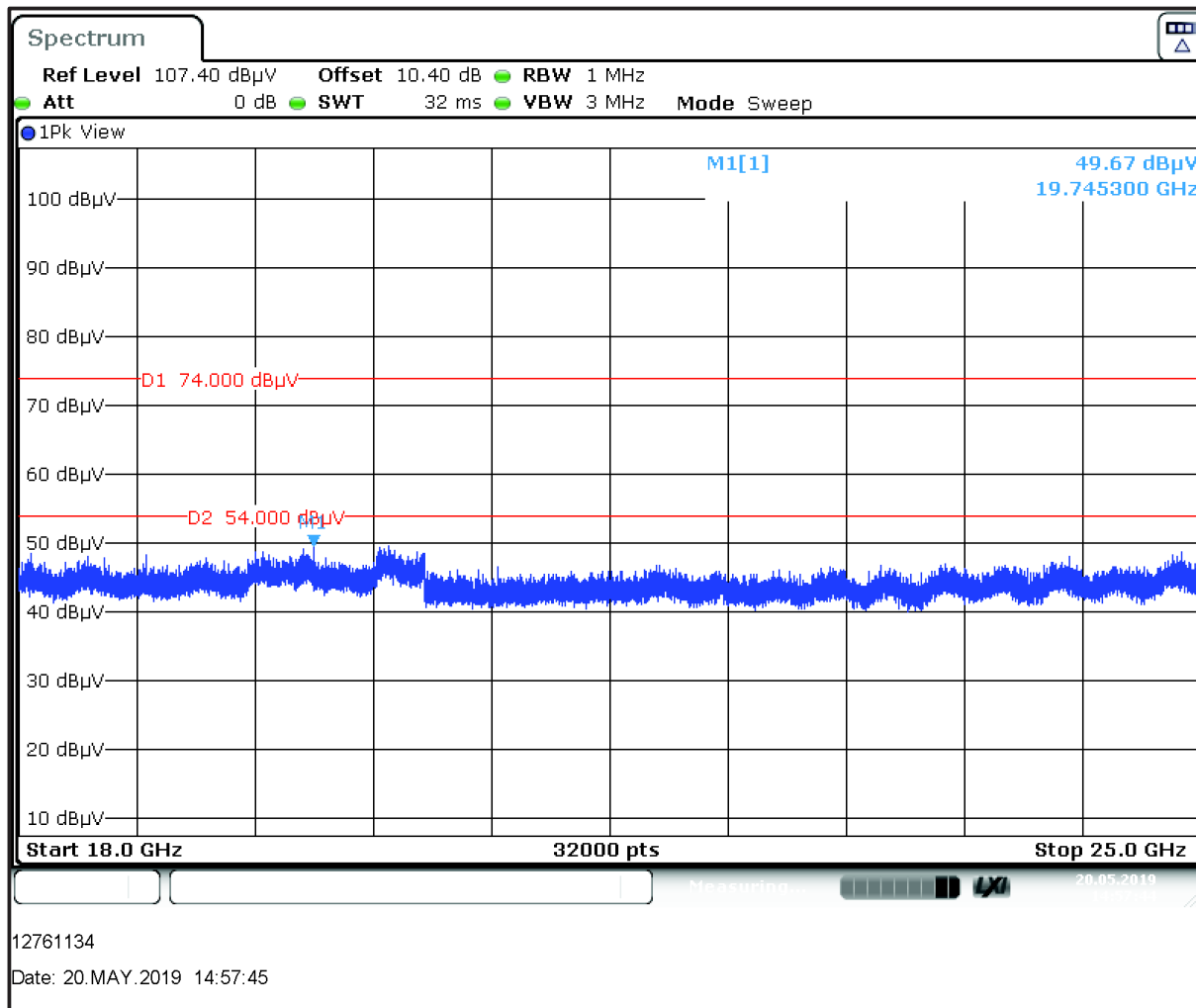
Plot: 18 GHz – 25GHz (Top Channel) with Peak detector
