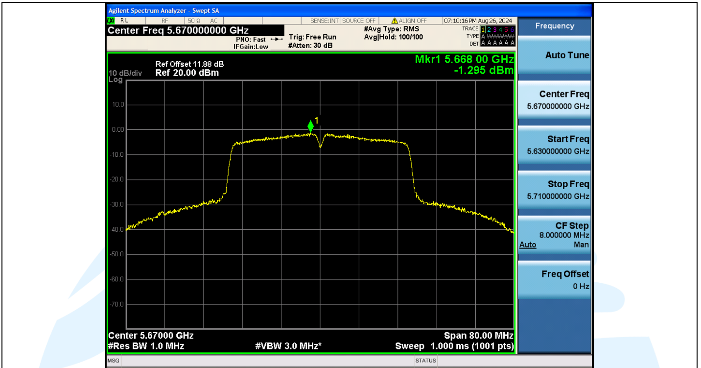
11N40MIMO-Ant2-5670-PASS
