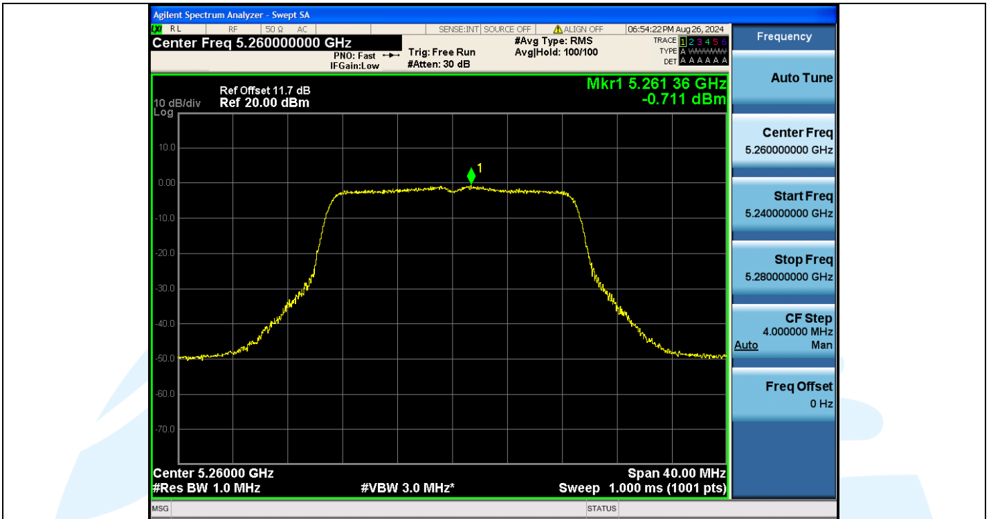
11N20MIMO-Ant2-5260-PASS
