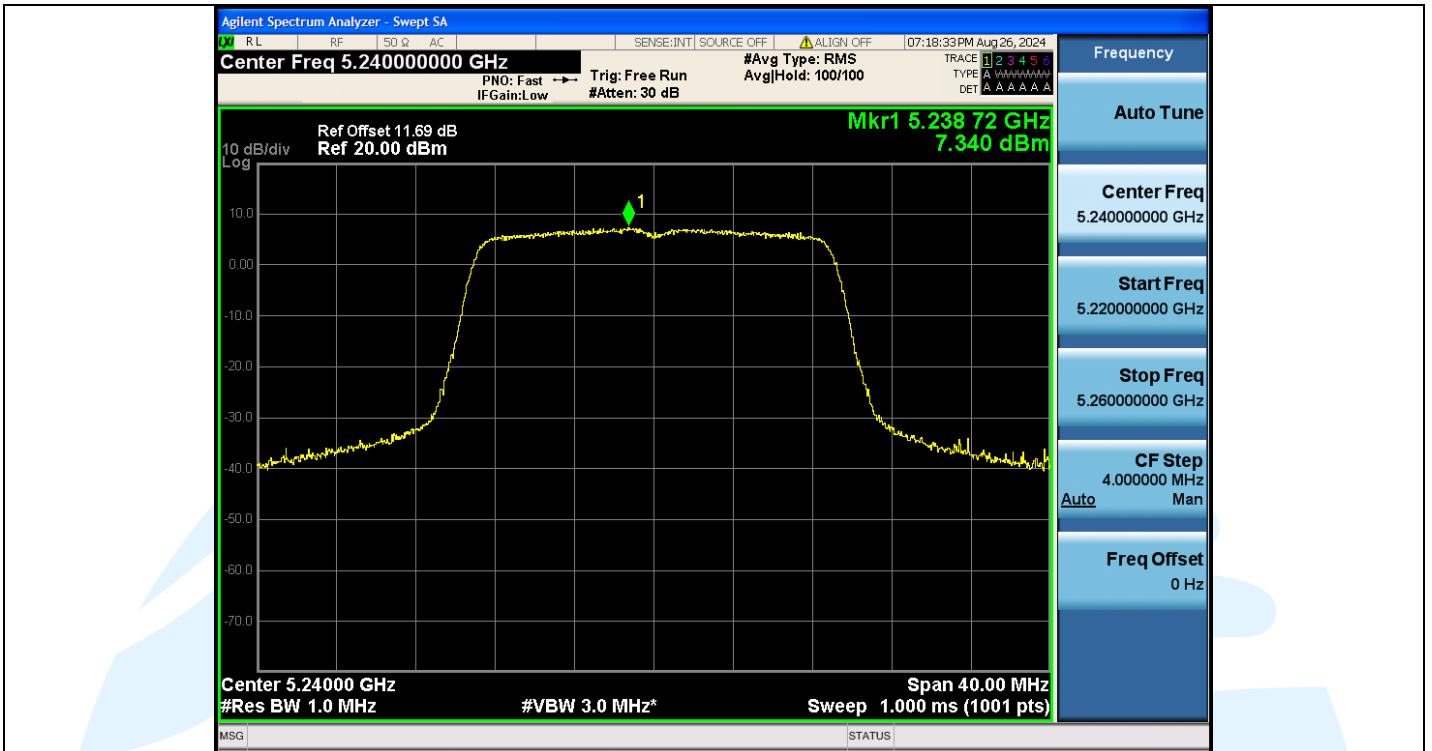
11AC20MIMO-Ant2-5240-PASS
