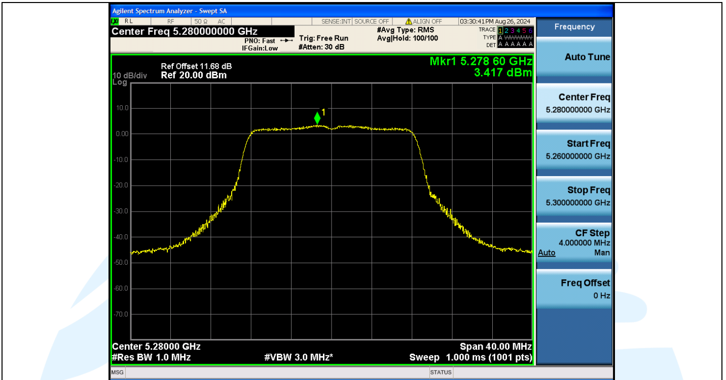
11A-Ant3-5280-PASS
