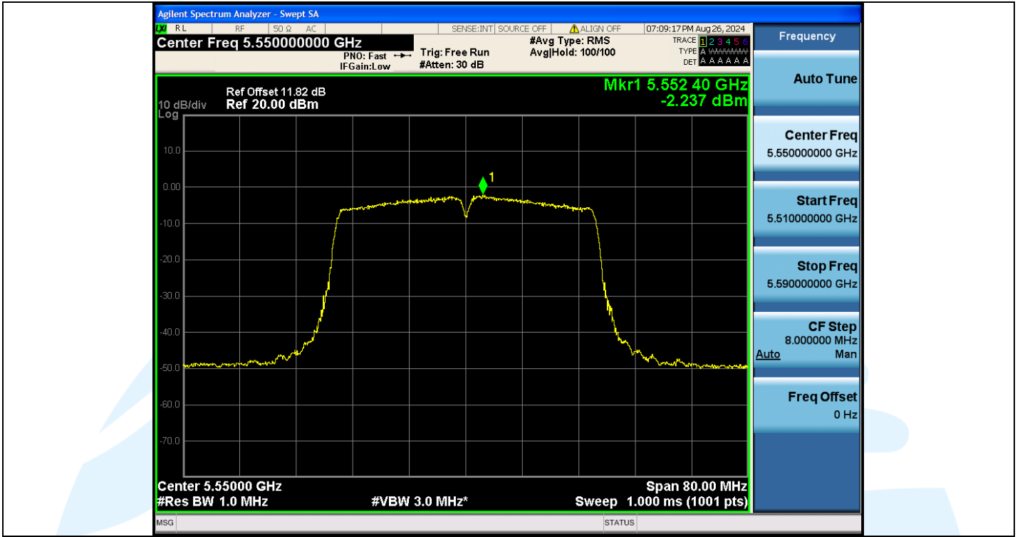
11N40MIMO-Ant2-5550-PASS
