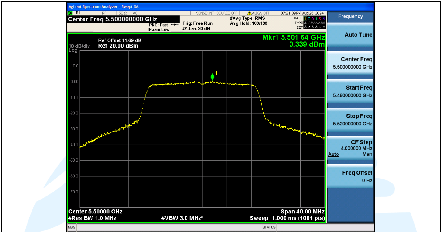
11AC20MIMO-Ant2-5500-PASS
