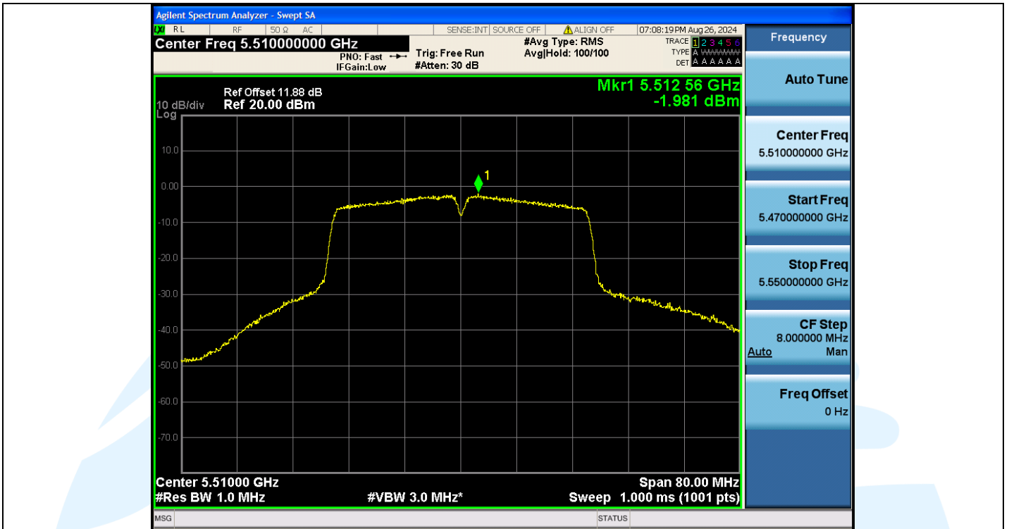
11N40MIMO-Ant2-5510-PASS
