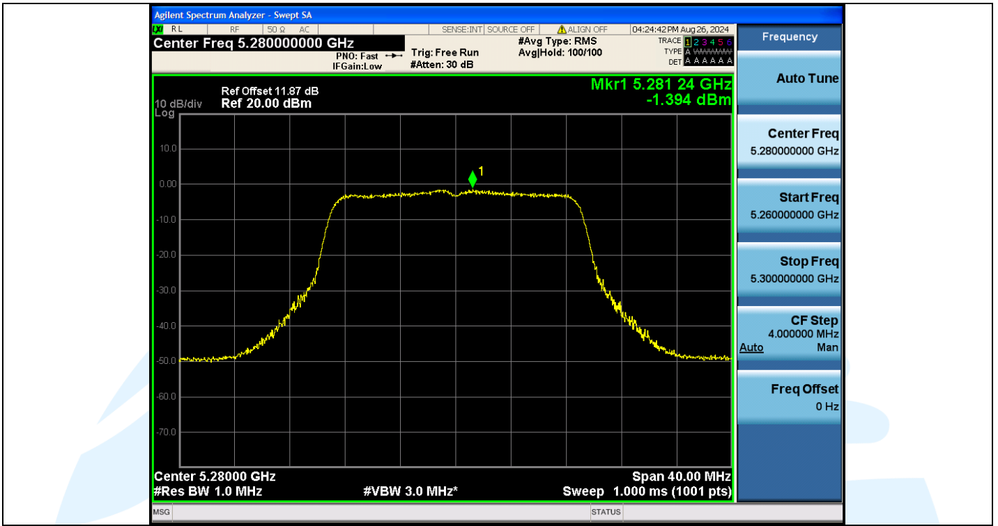
11AC20MIMO-Ant3-5280-PASS
