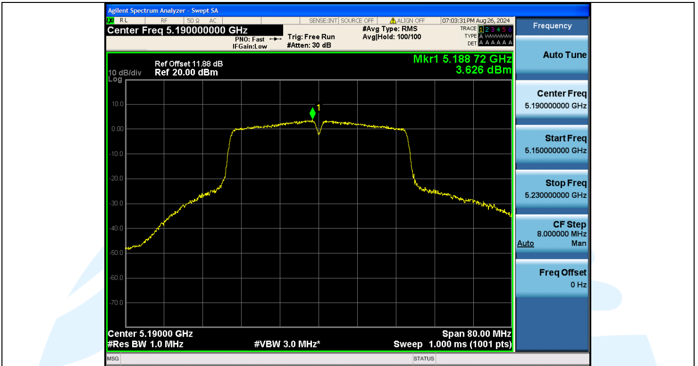
11N40MIMO-Ant2-5190-PASS
