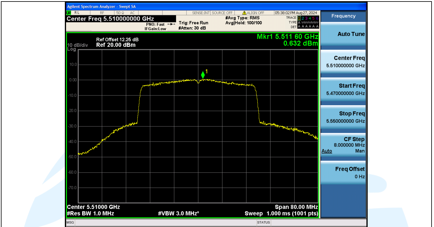
11AX40MIMO-Ant3-5510-PASS
