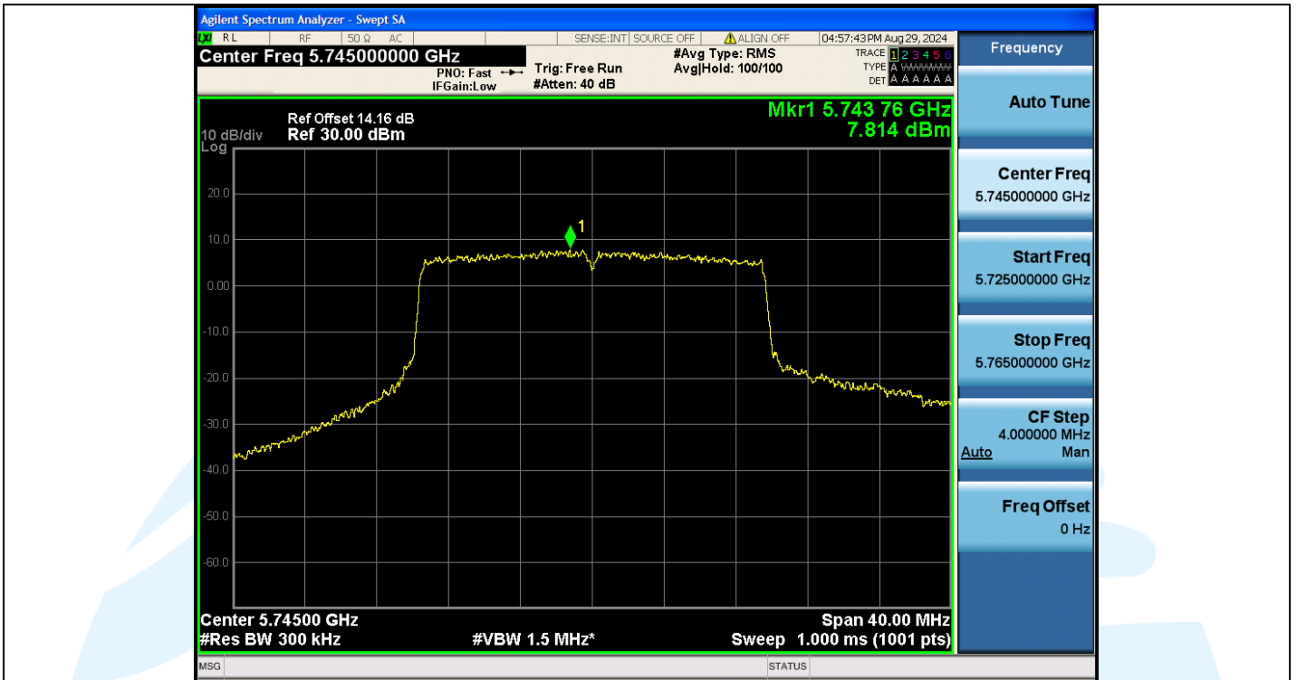
11AX20MIMO-Ant2-5745-PASS
