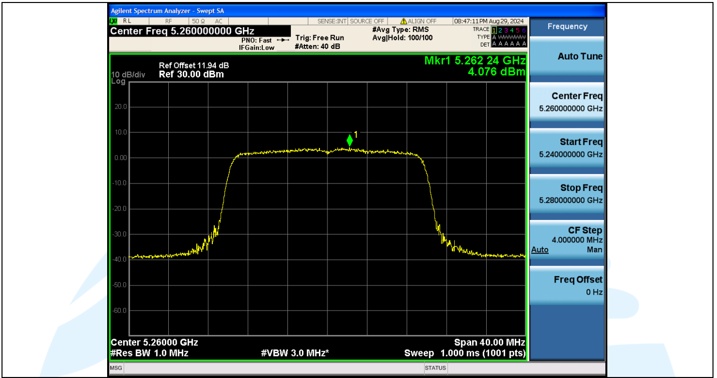
11AX20MIMO-Ant2-5260-PASS
