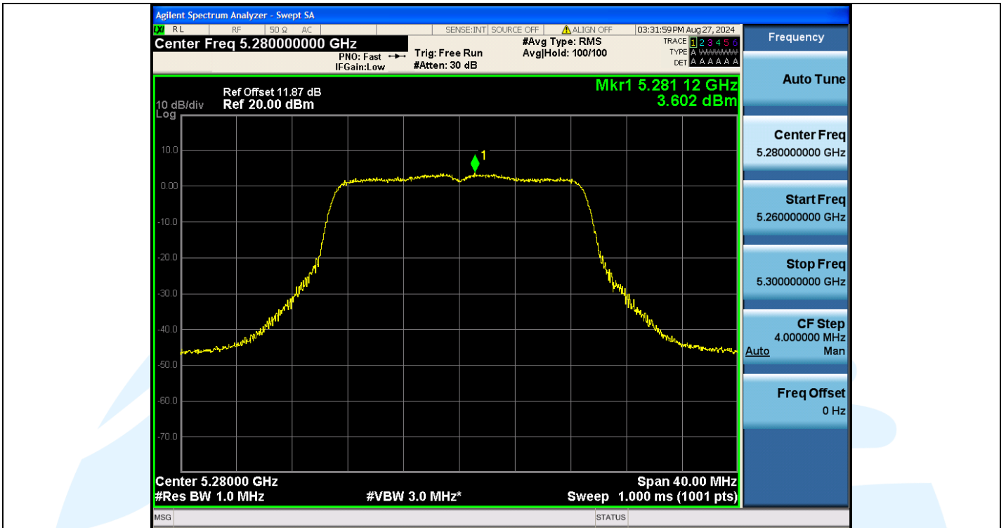
11N20MIMO-Ant3-5280-PASS
