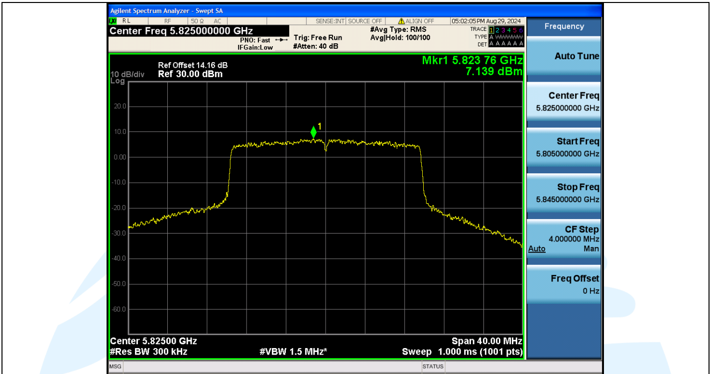
11AX20MIMO-Ant2-5825-PASS
