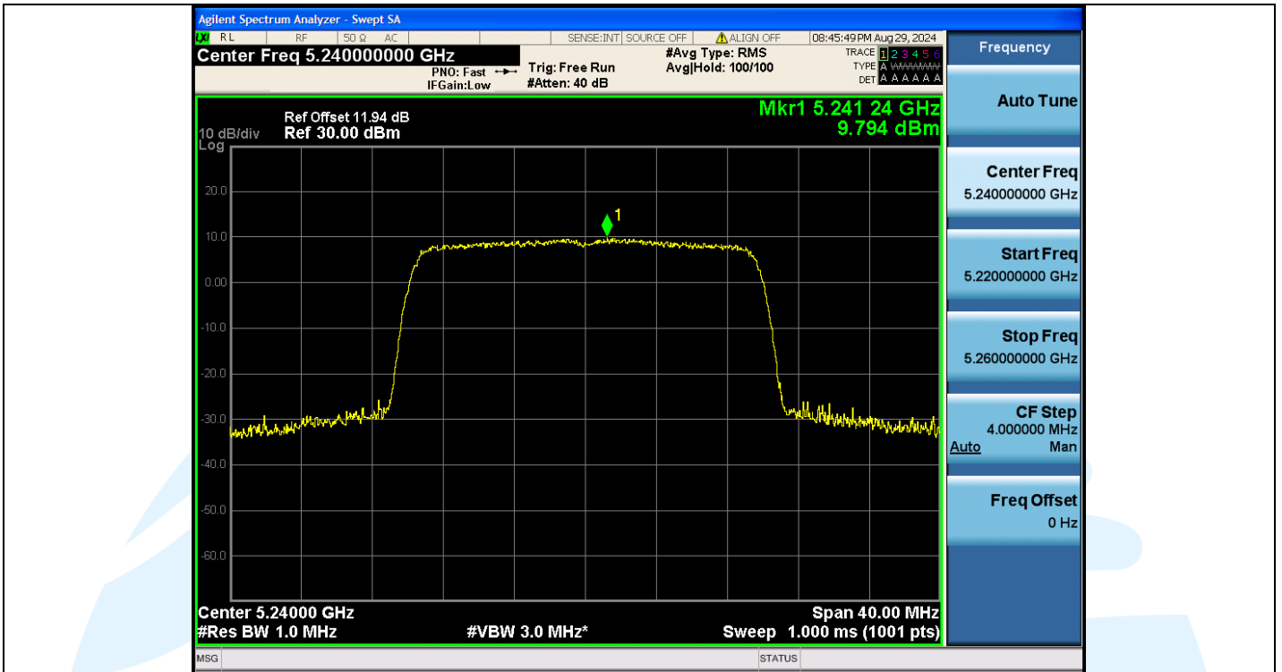
11AX20MIMO-Ant2-5240-PASS
