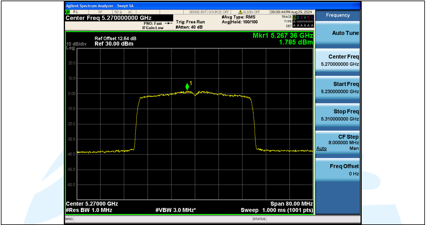
11AX40MIMO-Ant2-5270-PASS
