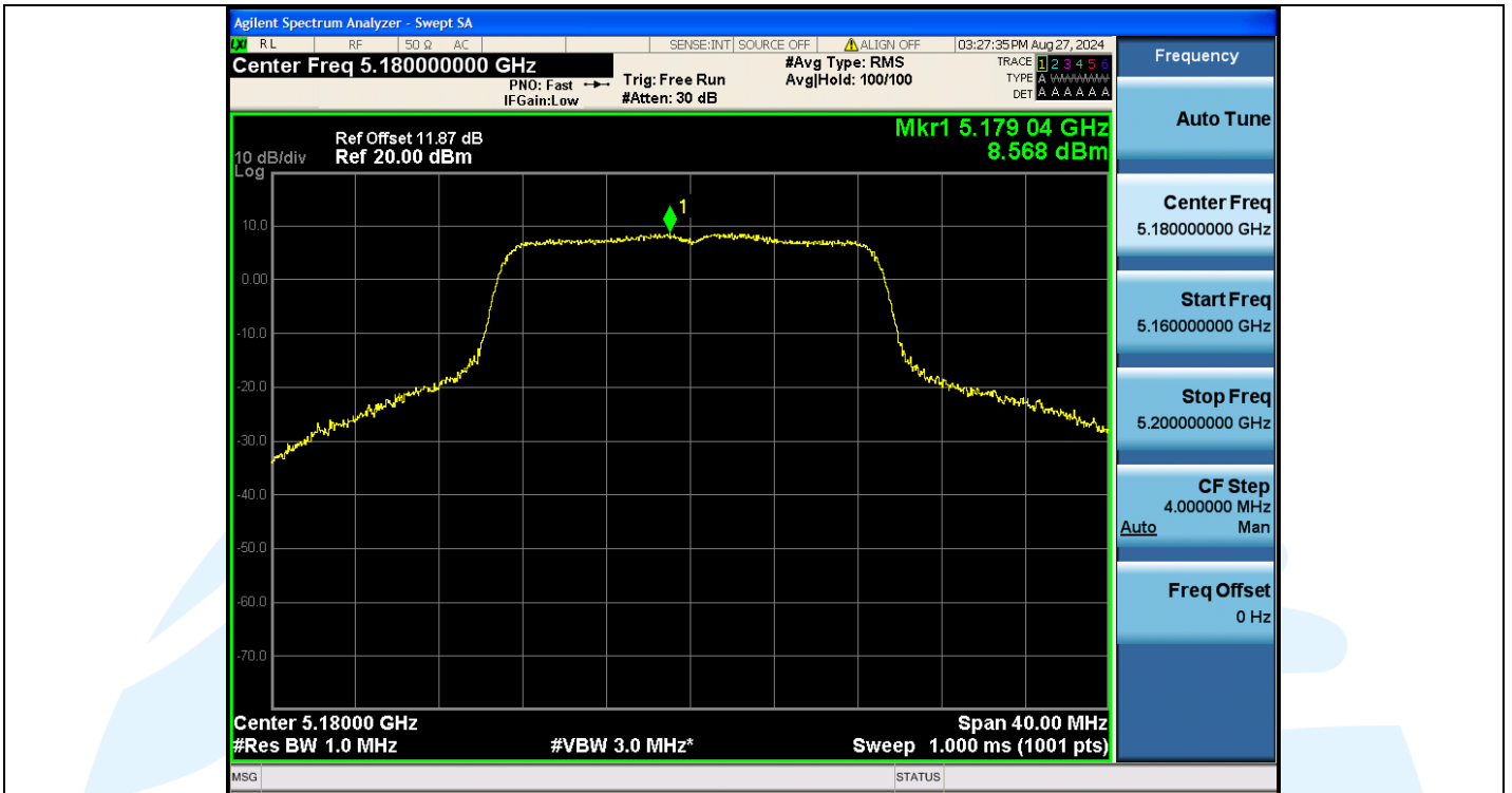
11N20MIMO-Ant3-5180-PASS
