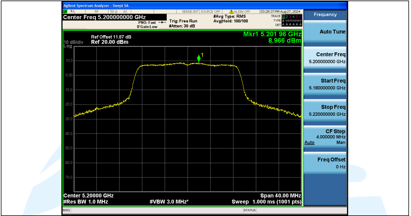
11N20MIMO-Ant3-5200-PASS
