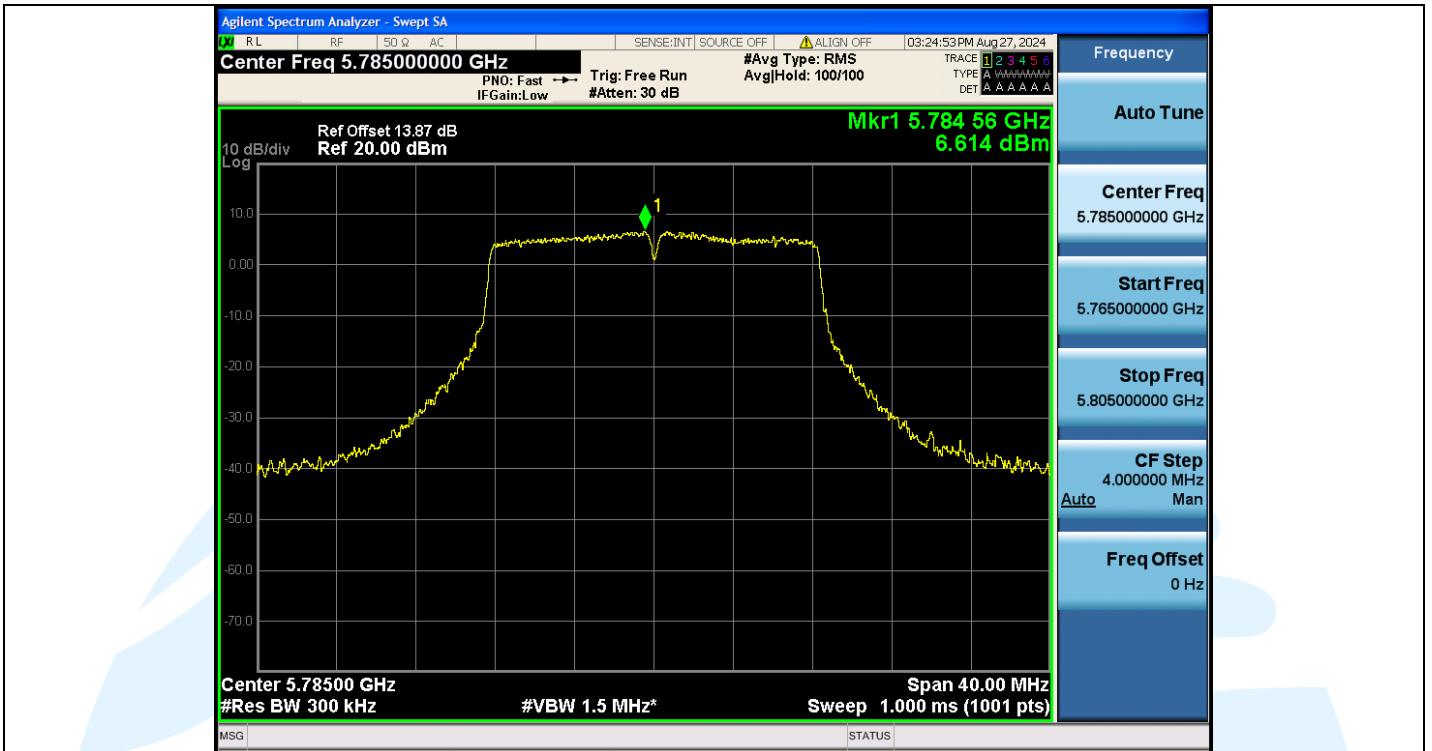
11A-Ant3-5785-PASS
