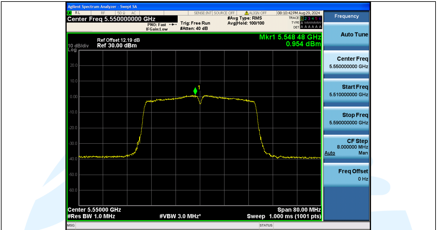
11N40MIMO-Ant2-5550-PASS
