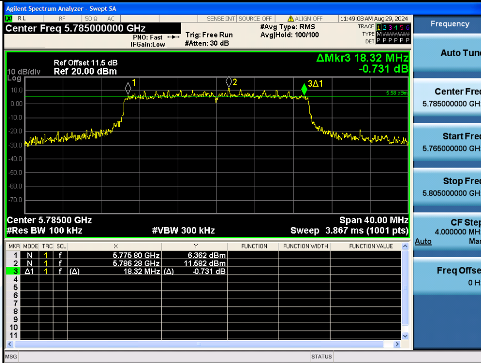
11AX20MIMO-Ant3-5785-PASS
