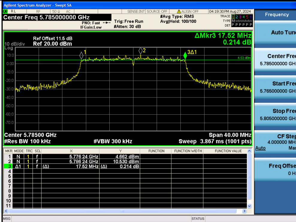
11AC20MIMO-Ant3-5785-PASS
