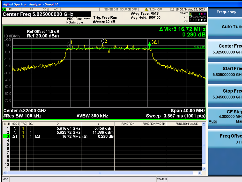
11AC20MIMO-Ant3-5825-PASS
