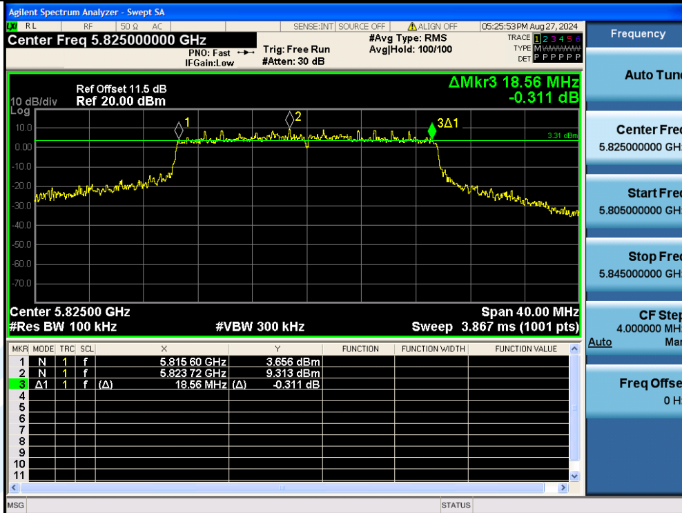
11AX20MIMO-Ant3-5825-PASS
