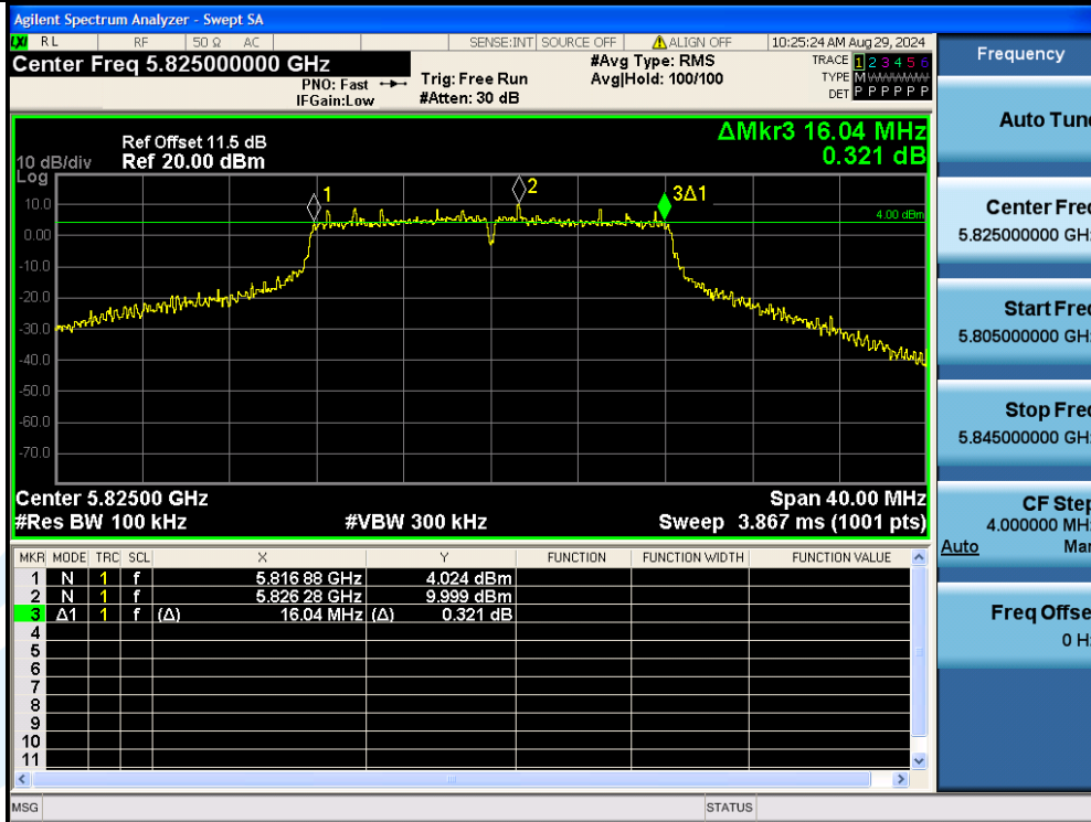
11A-Ant3-5825-PASS
