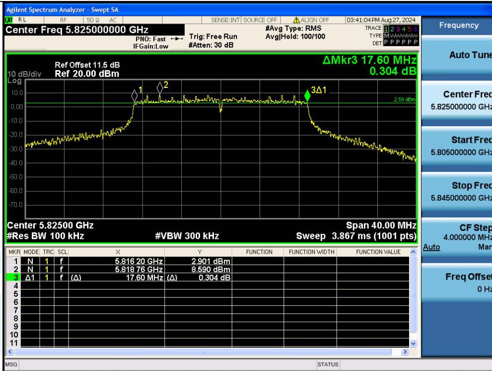
11N20MIMO-Ant3-5825-PASS
