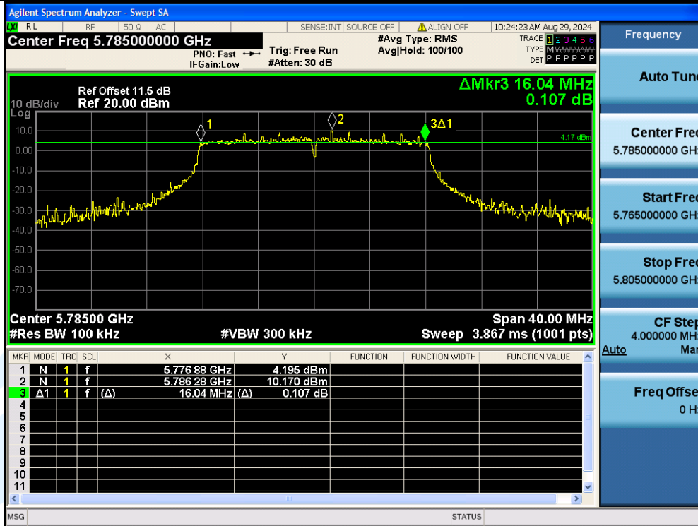
11A-Ant3-5785-PASS
