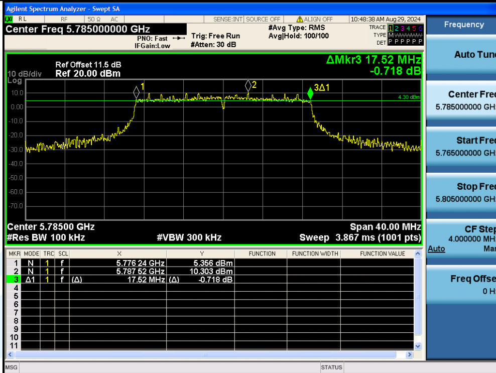
11N20MIMO-Ant3-5785-PASS
