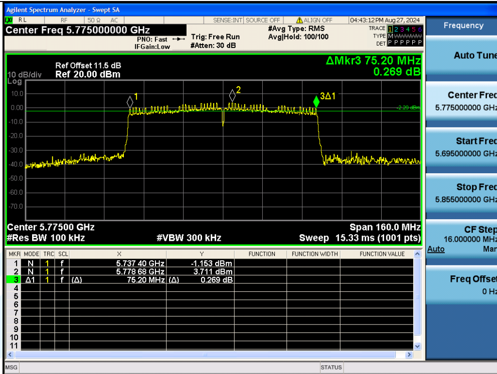
11AC80MIMO-Ant3-5775-PASS
