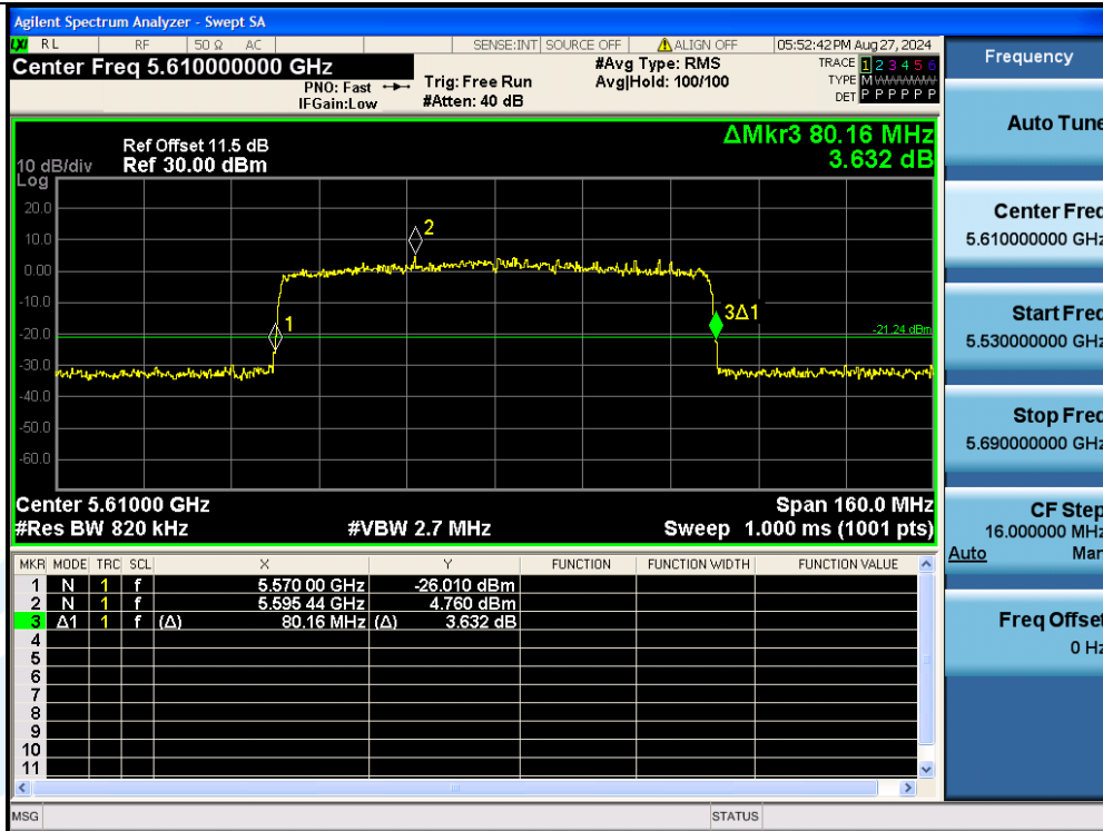
11AX80MIMO-Ant3-5610
