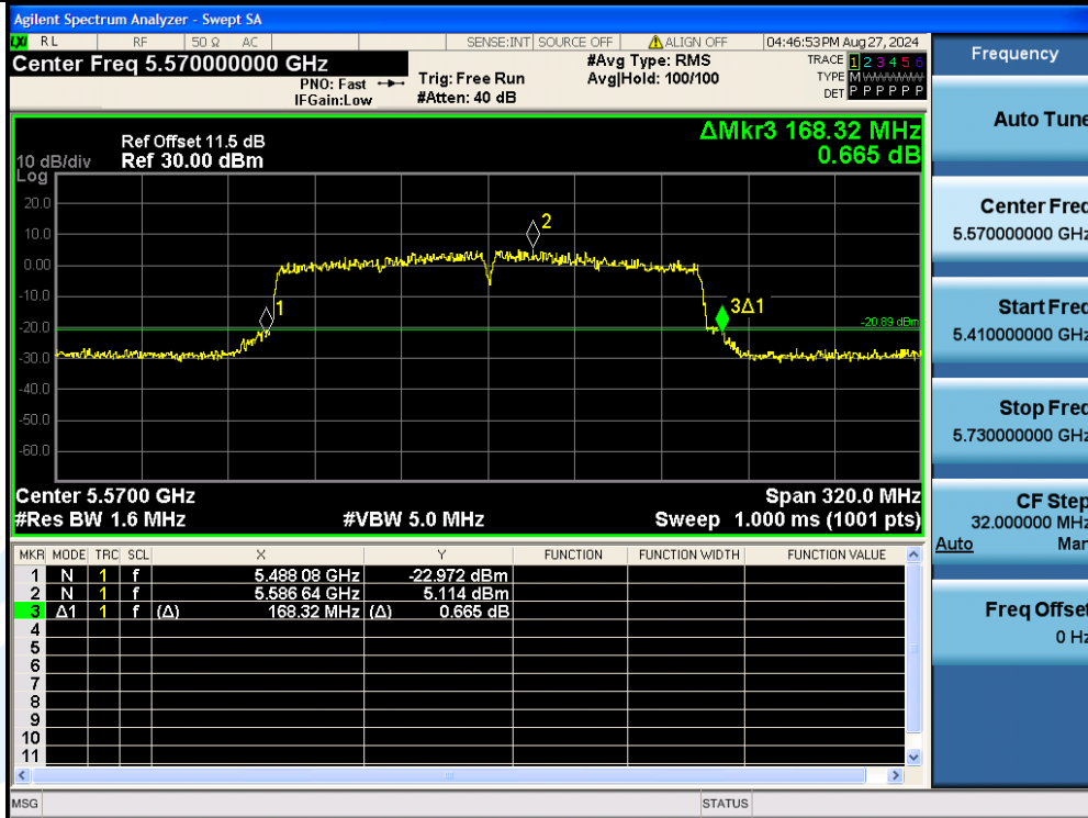
11AC160MIMO-Ant3-5570
