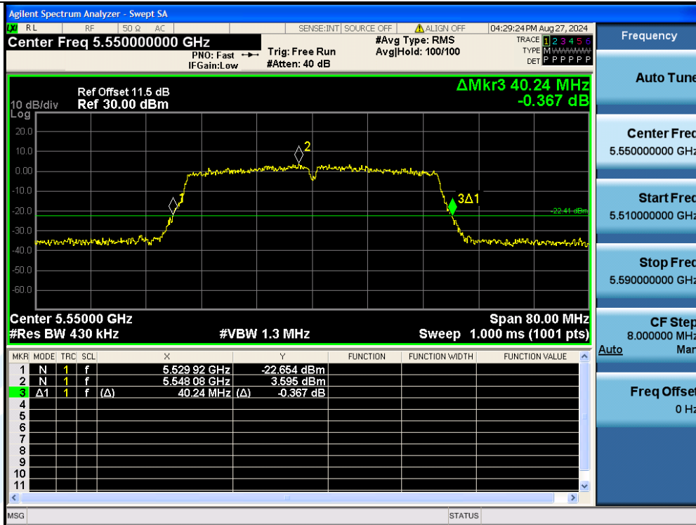
11AC40MIMO-Ant3-5550
