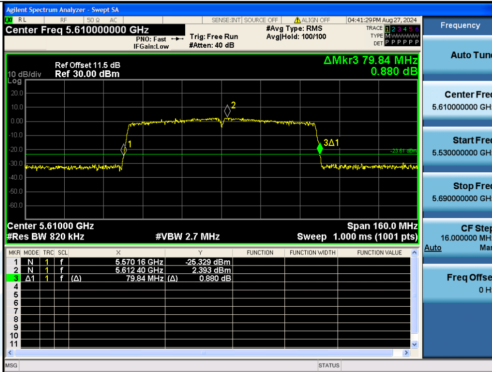
11AC80MIMO-Ant3-5610
