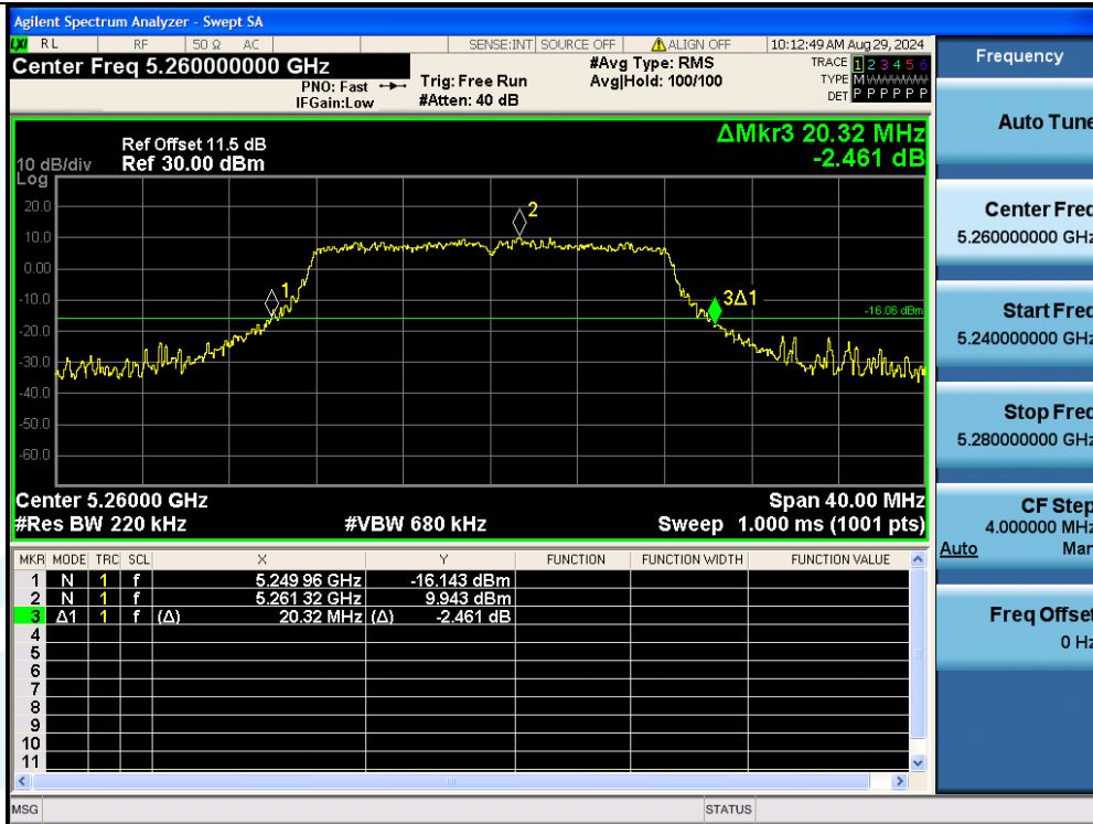
11A-Ant3-5260
