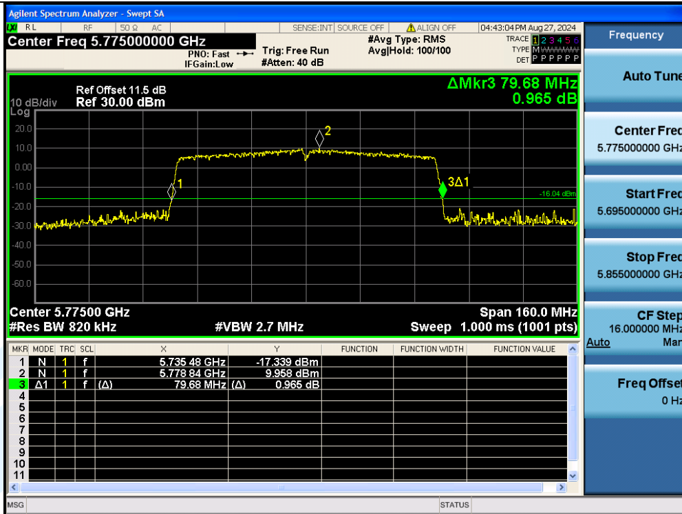
11AC80MIMO-Ant3-5775
