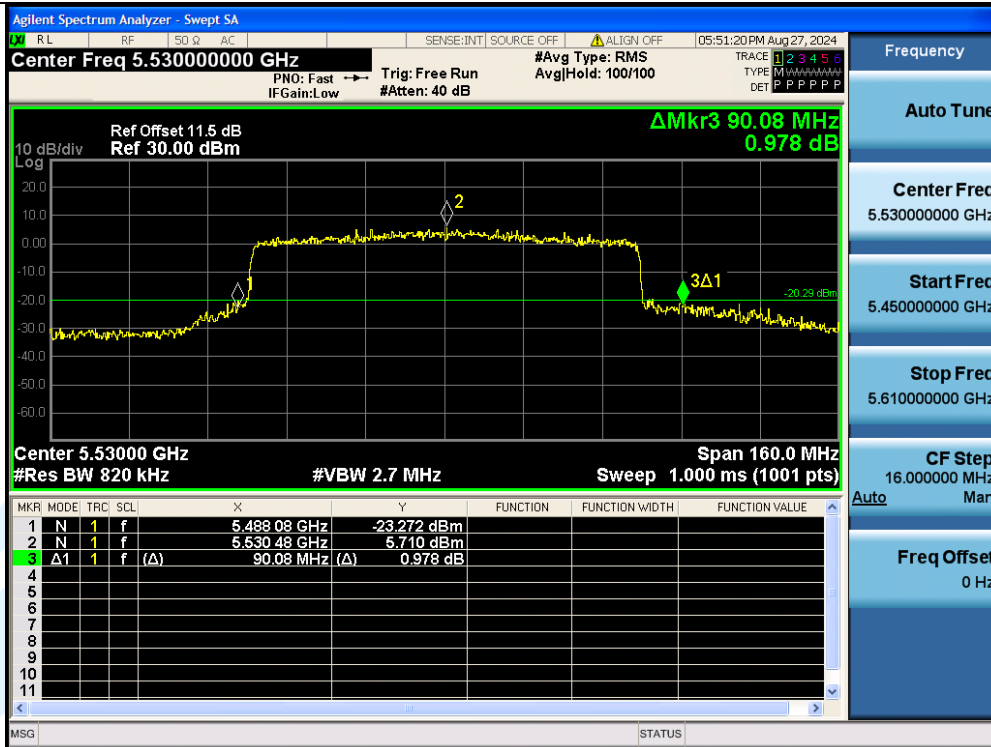
11AX80MIMO-Ant3-5530
