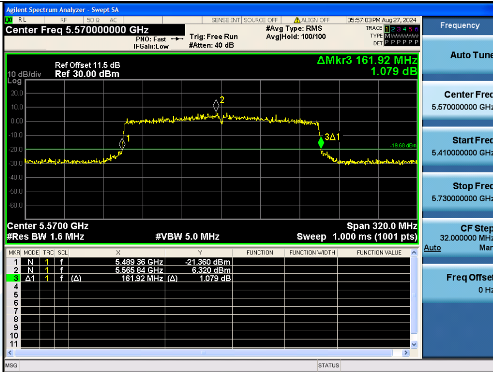
11AX160MIMO-Ant3-5570
