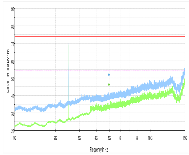
Figure 8.3-11: Radiated spurious emissions for high channel
