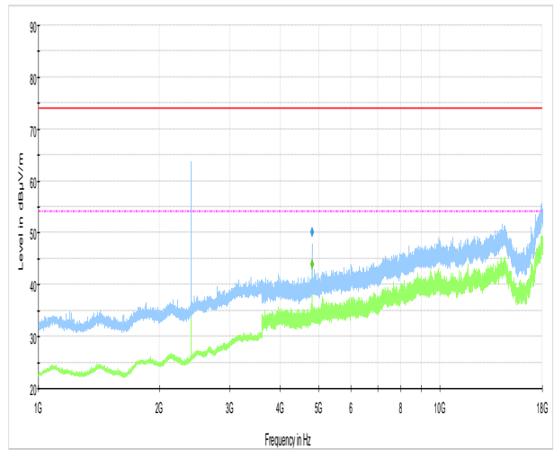
Figure 8.3-7: Radiated spurious emissions for low channel
