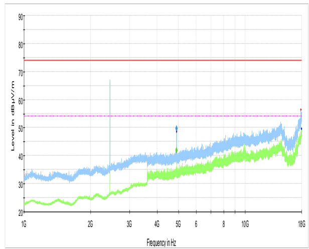
Figure 8.3-9: Radiated spurious emissions for mid channel
