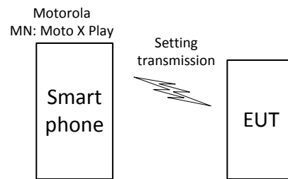
Figure 3.6-1: Setup diagram
