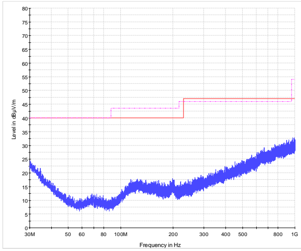
Figure 8.3-10: Radiated spurious emissions for high channel
