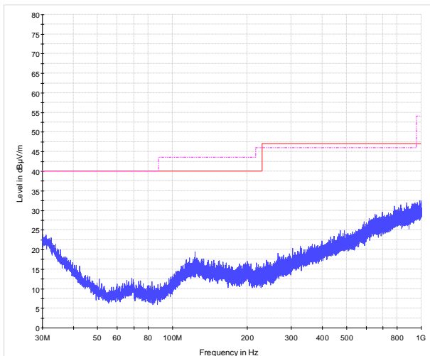
Figure 8.3-8: Radiated spurious emissions for mid channel
