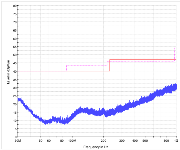
Figure 8.3-6: Radiated spurious emissions for low channel
