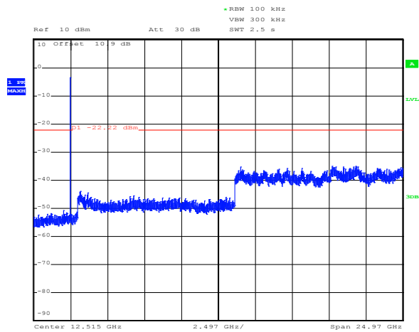
Figure 8.3-3: Conducted spurious emissions for low channel
