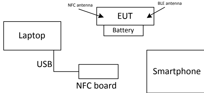
Figure 3.6-1: Setup diagram
