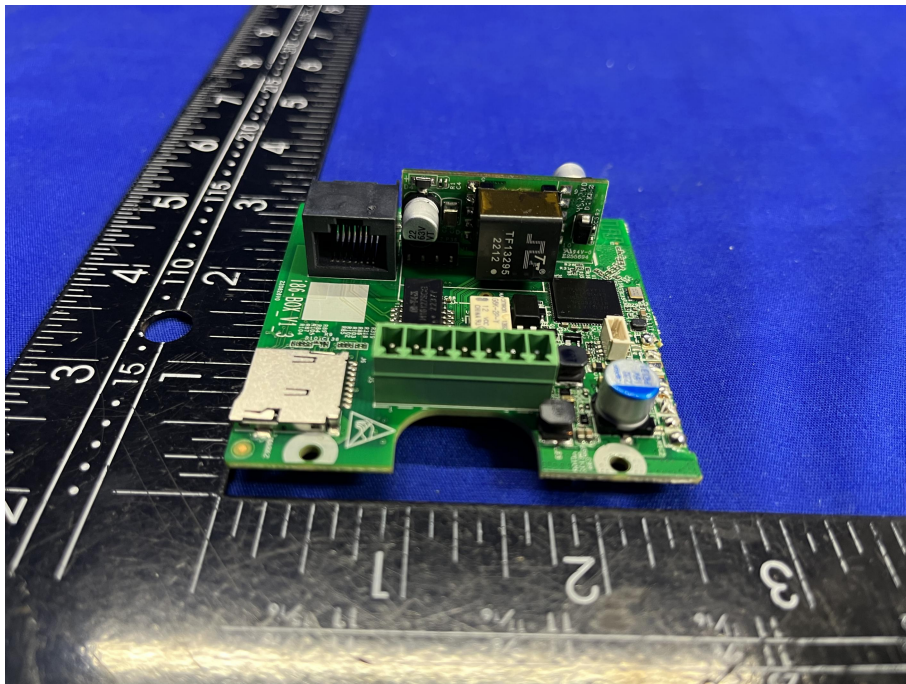
EUT View 10
