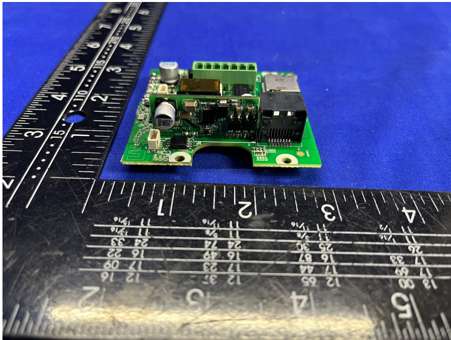
EUT View 9
